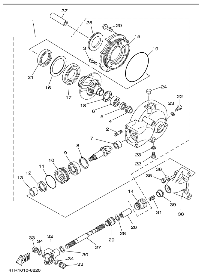
FIG.22 DRIVE SHAFT
