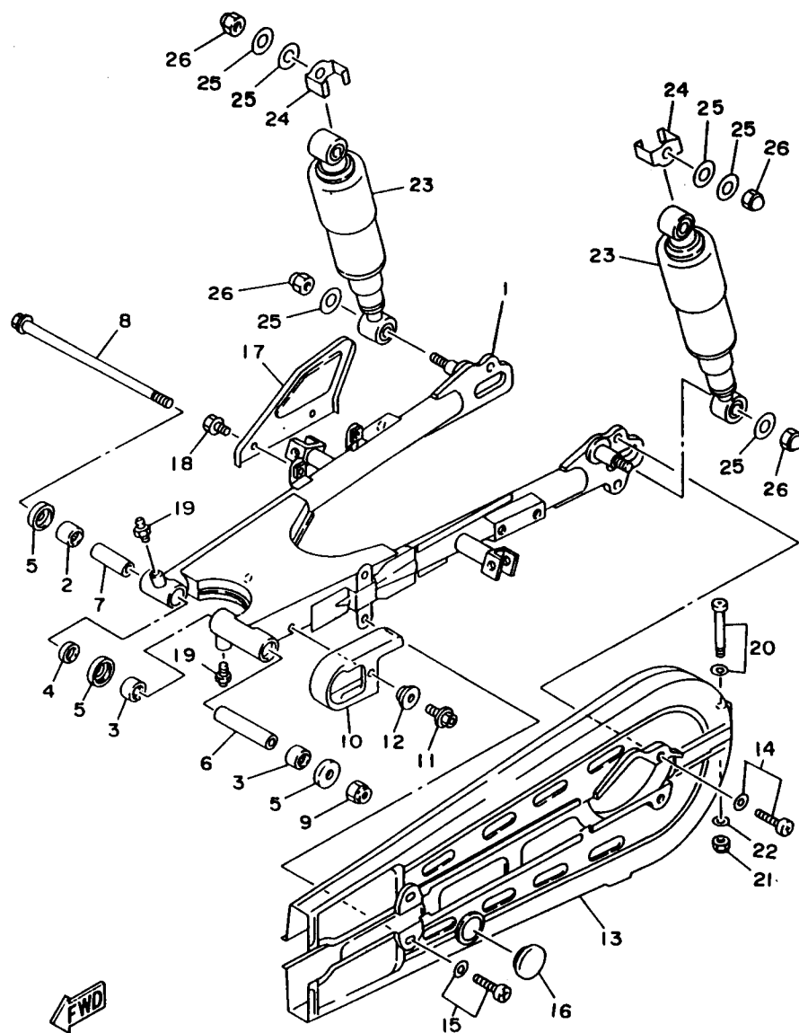
FIG. 21 REAR ARM. SUSPENSION
