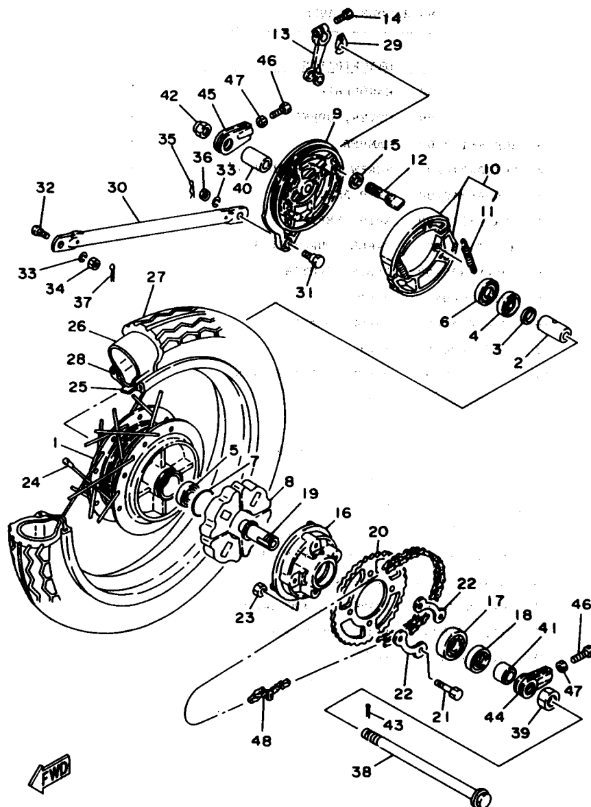
FIG. 27 REAR WHEEL
