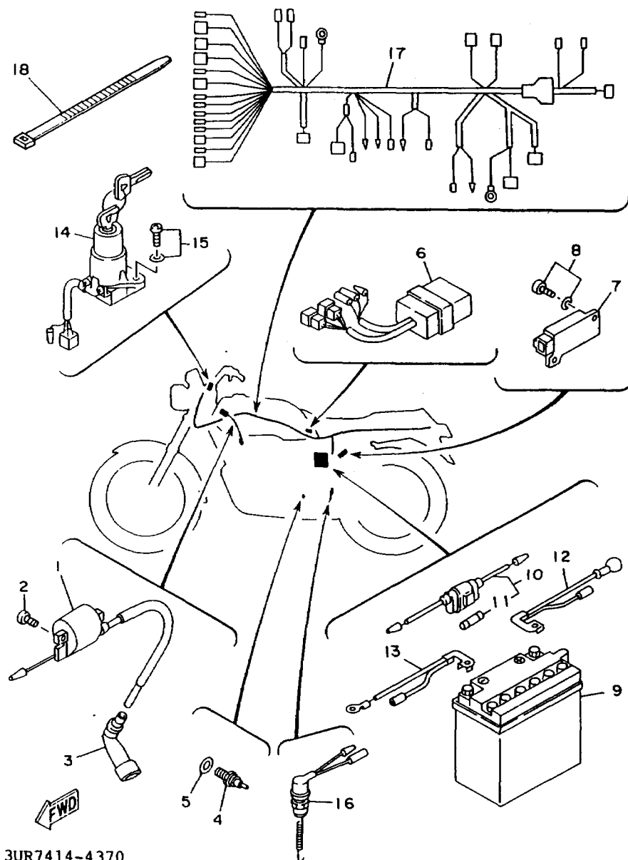
FIG. 37 ELECTRICAL 1
