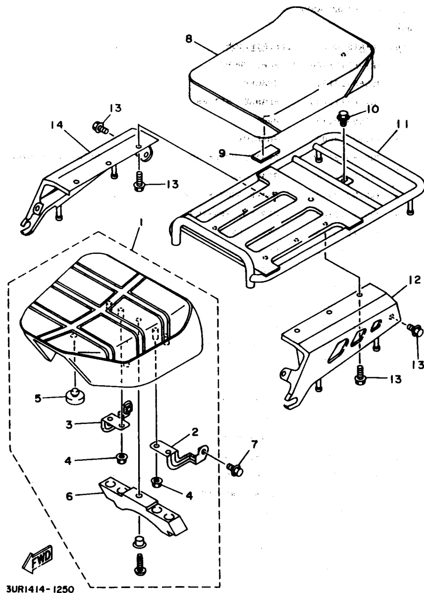
FIG. 25 SEAT. CARRIER
