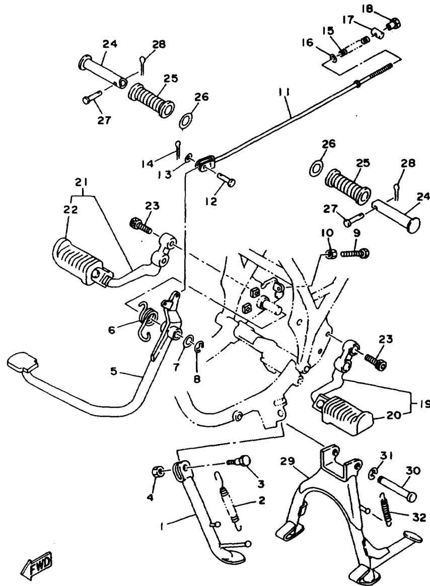
FIG. 29 STAND. FOOTREST
