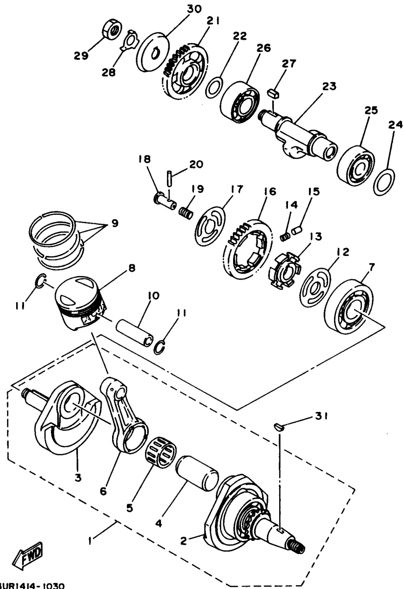
FIG. 3 CRANKSHAFT. PISTON
