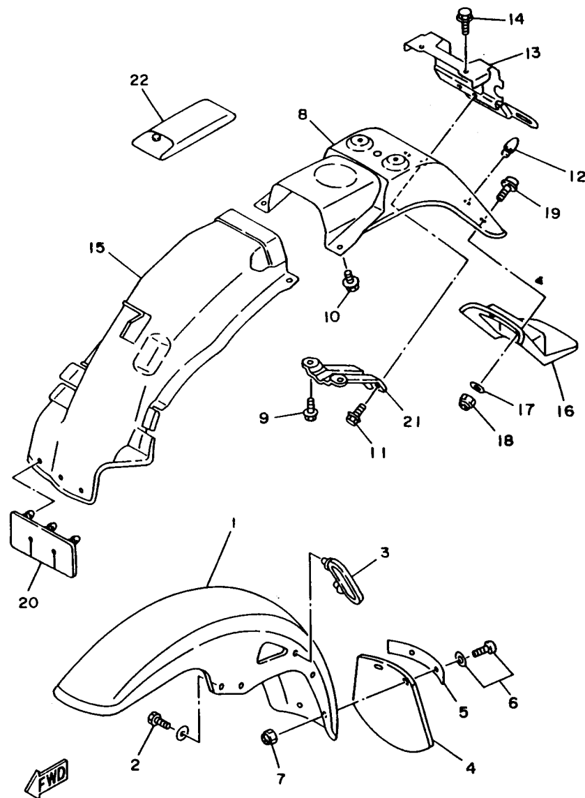
FIG. 19 FRONT FENDER
