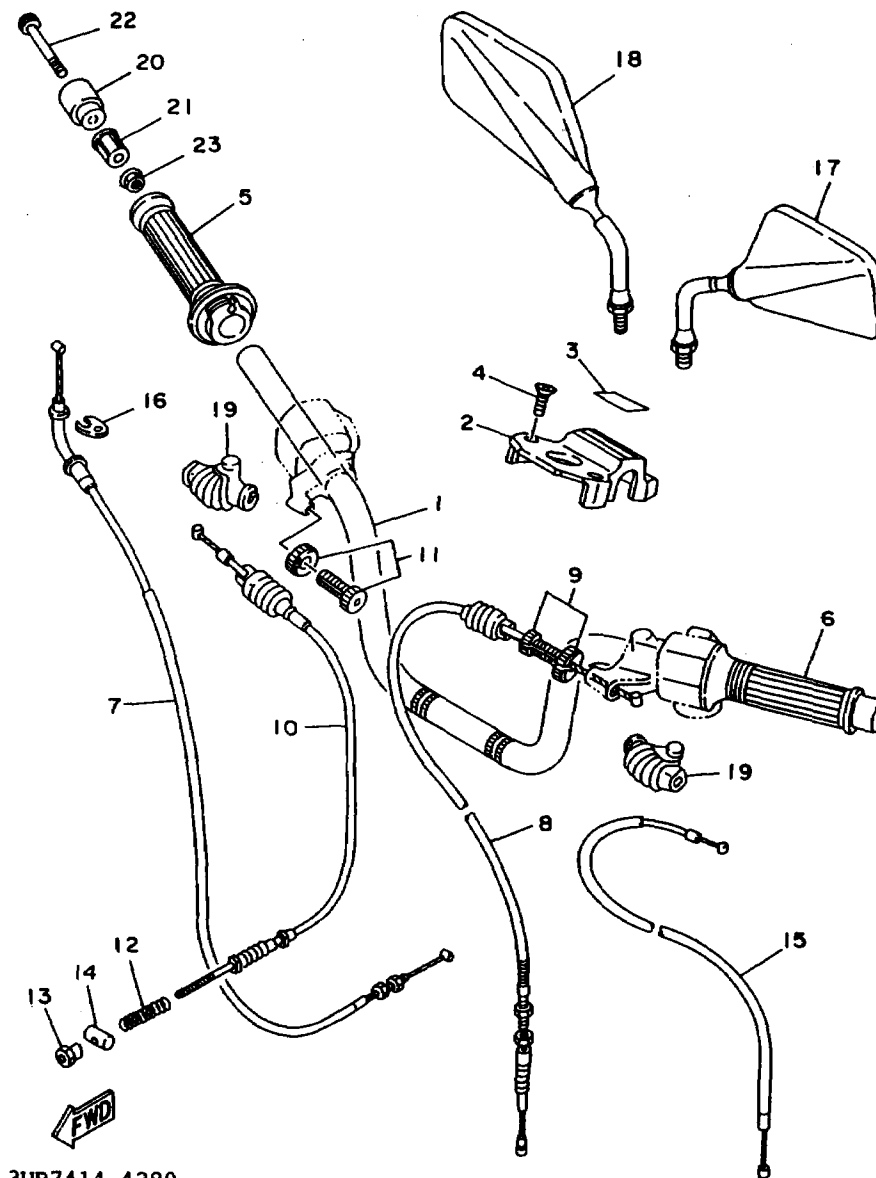
FIG. 28 STEERING HANDLE. CABLE
