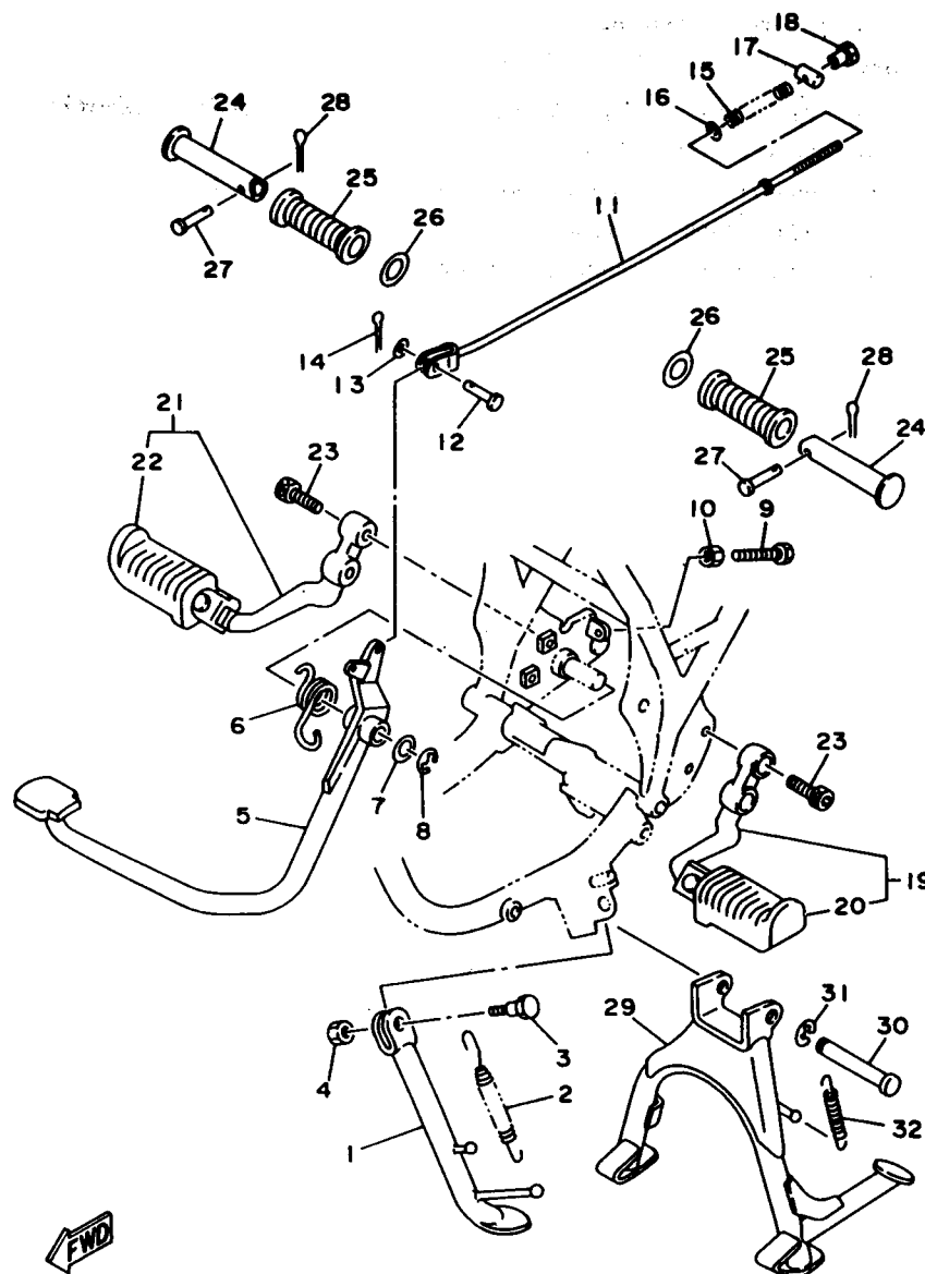
FIG. 29 STAND. FOOTREST
