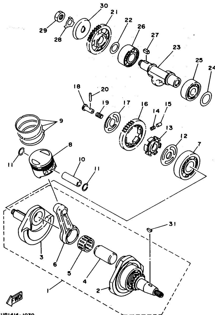
FIG. 3 CRANKSHAFT. PISTON
