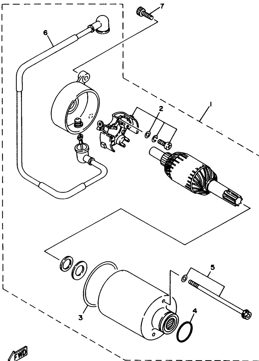
FIG. 31 STARTING MOTOR
