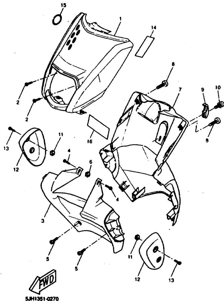
FIG 28 LEG SHIELD
