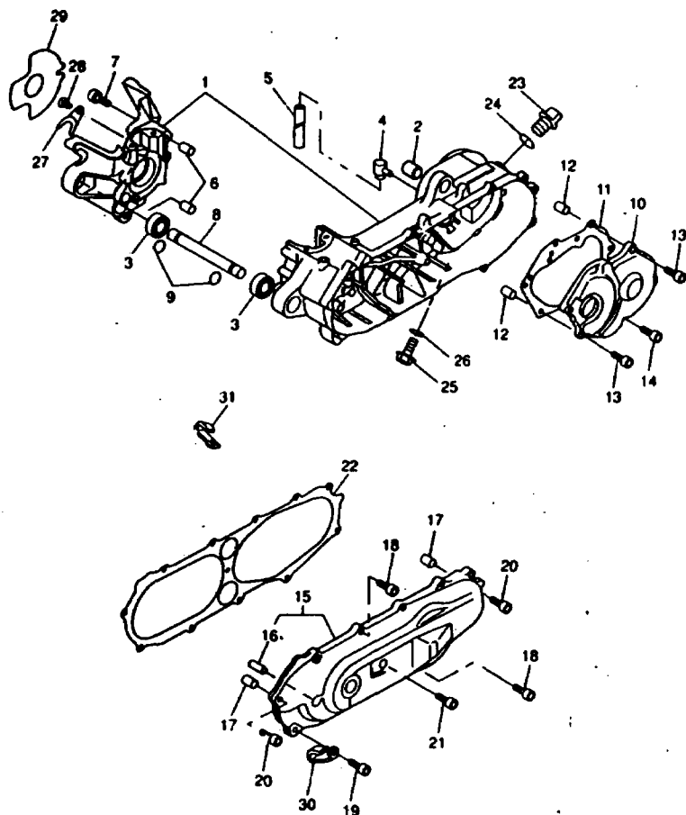
FIG 8 CRANKCASE
