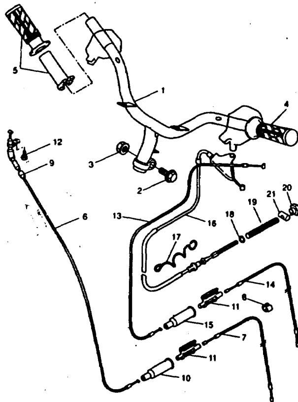
FIG 23 STEERING HANDLE CABLE
