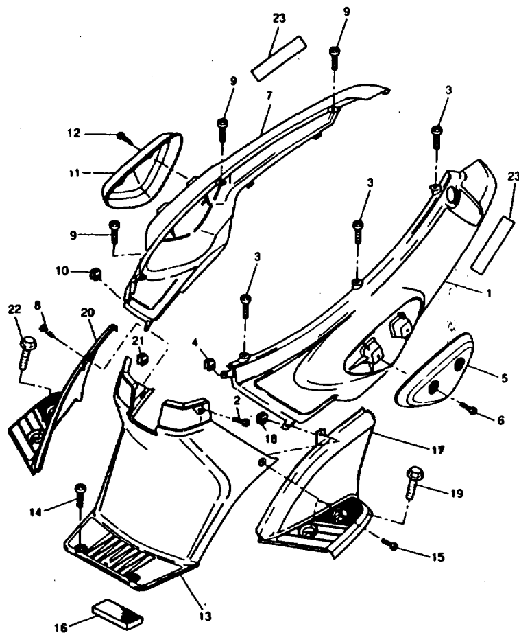
FIG 14 SIDE COVER
