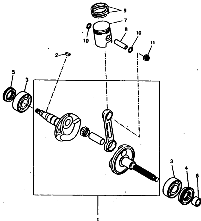
FIG 2 CRANKSHAFT, PISTON
