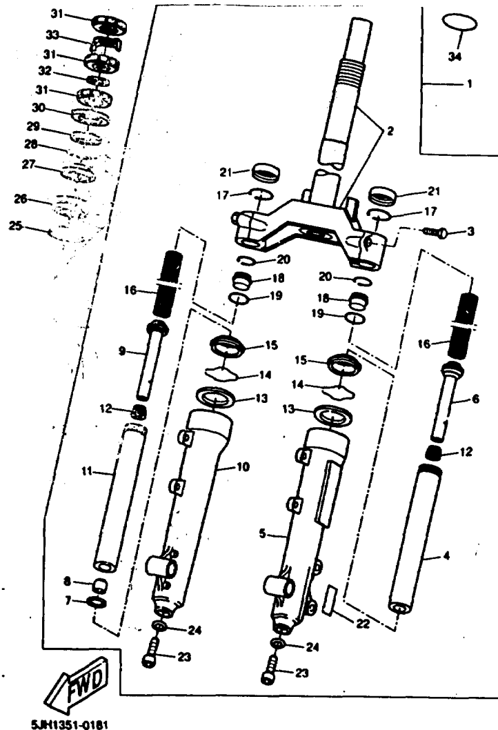
FIG 17 FRONT FORK
