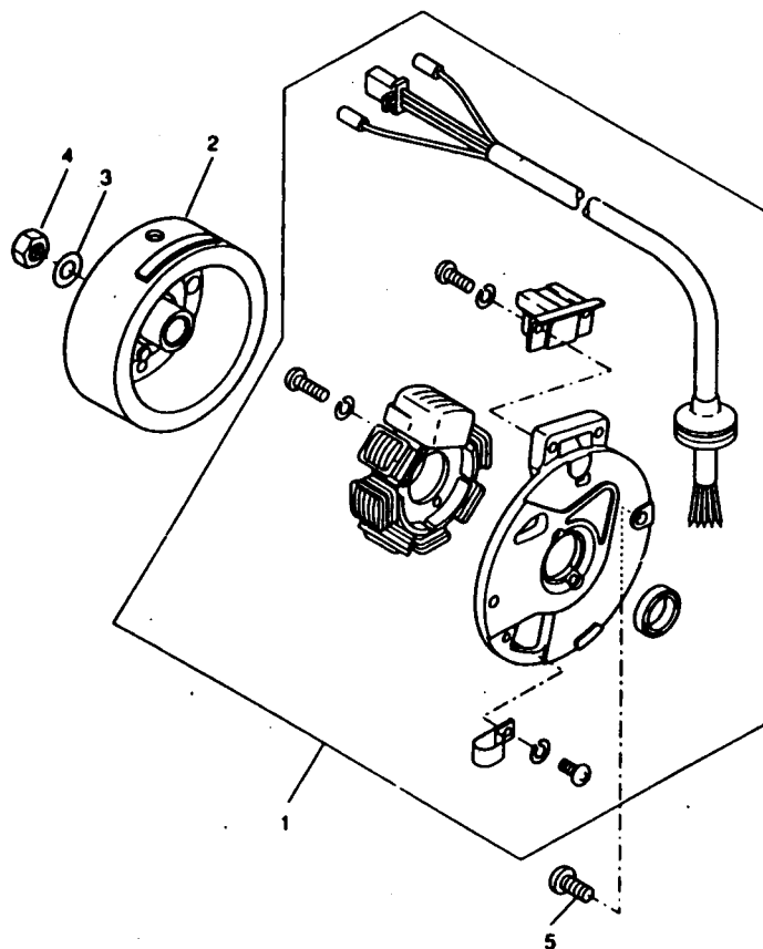
FIG 28 GENERATOR
