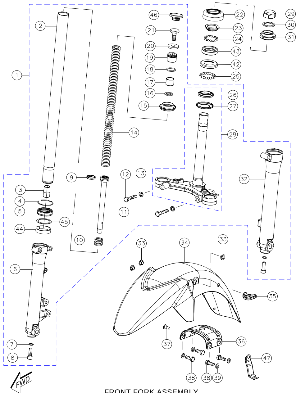
FRONT FORK ASSEMBLY
