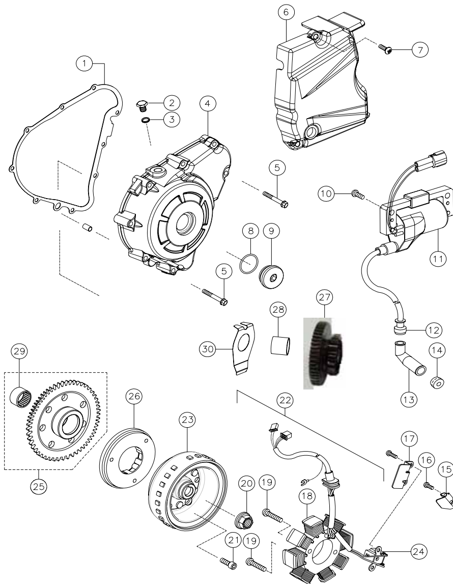
MAGNETO &amp; IGNITION COIL ASSEMBLY
