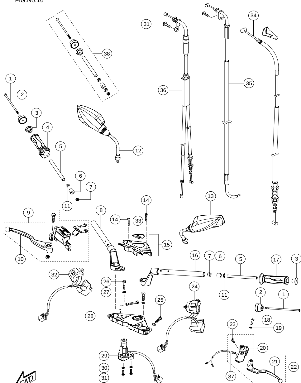
HANDLE BAR &amp; CABLE ASSY.
