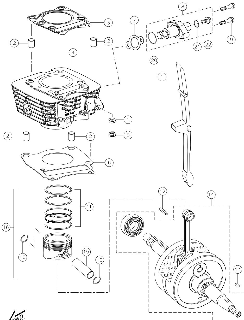
CYLINDER BLOCK & CRANK SHAFT ASSY.
