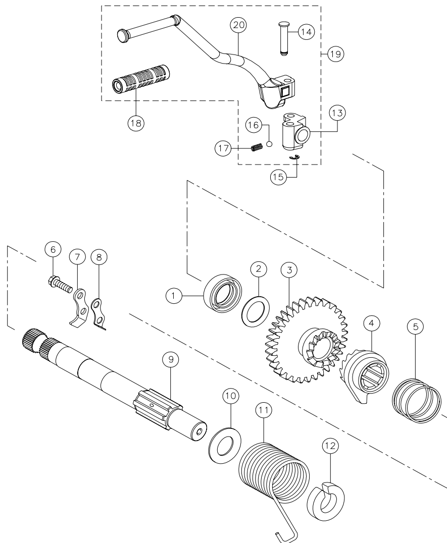
KICK STARTER ASSEMBLY
