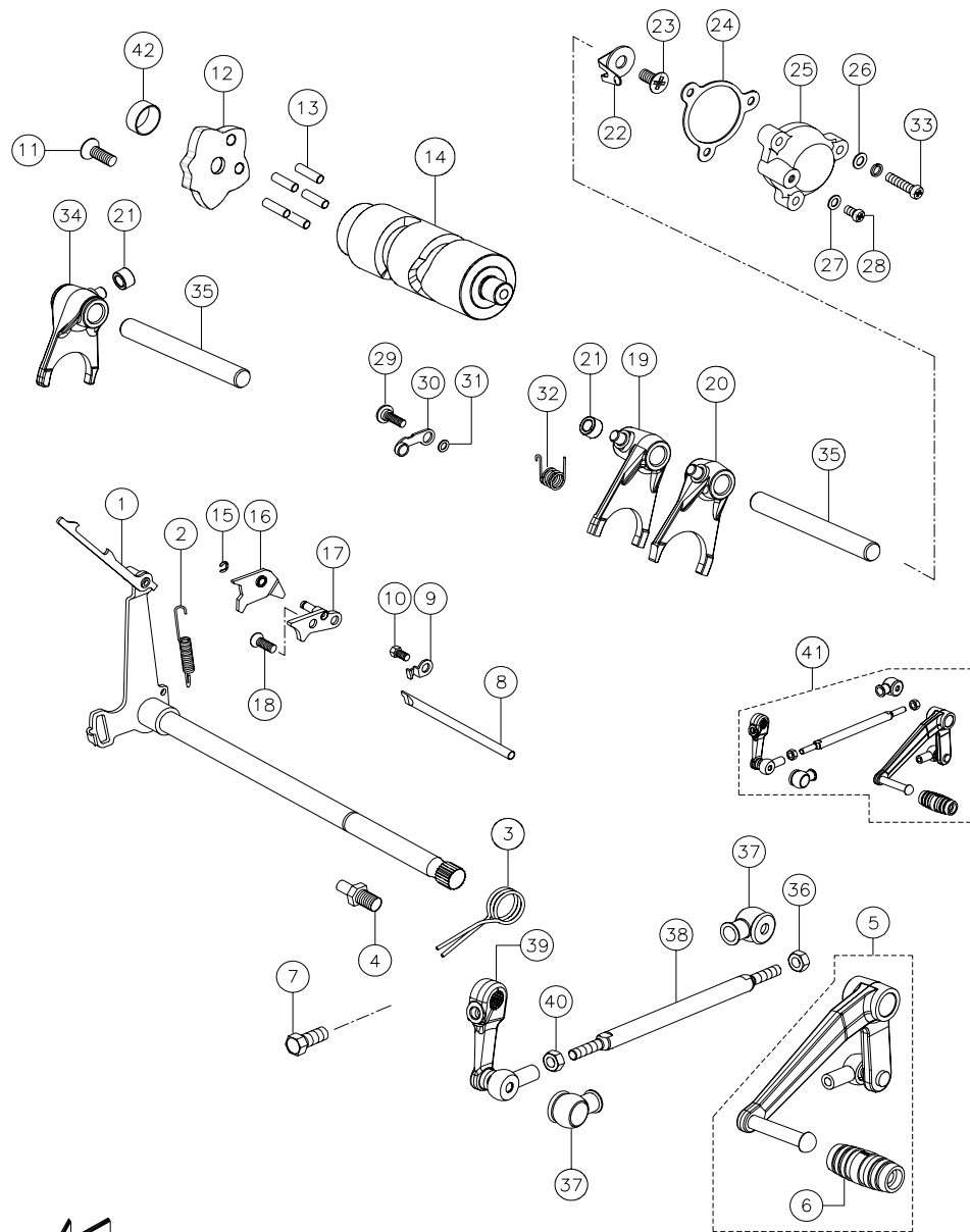
GEAR SHIFT MECHANISM ASSEMBLY
