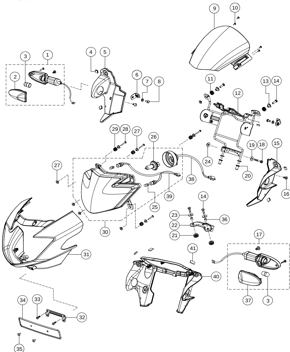
HEAD LAMP ASSY. &amp; TSL LH, RH
