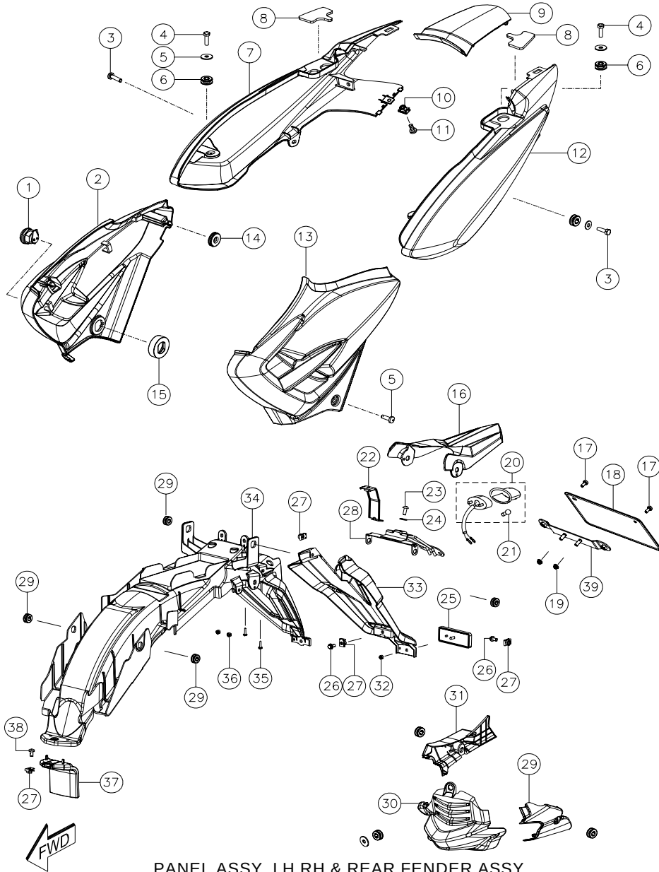
PANEL ASSY. LH,RH &amp; REAR FENDER ASSY.
