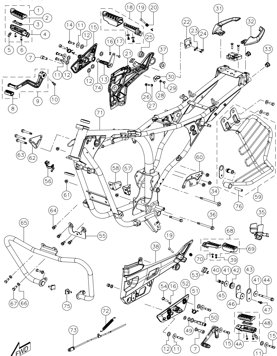
FRAME &amp; SAREE GUARD ASSEMBLY
