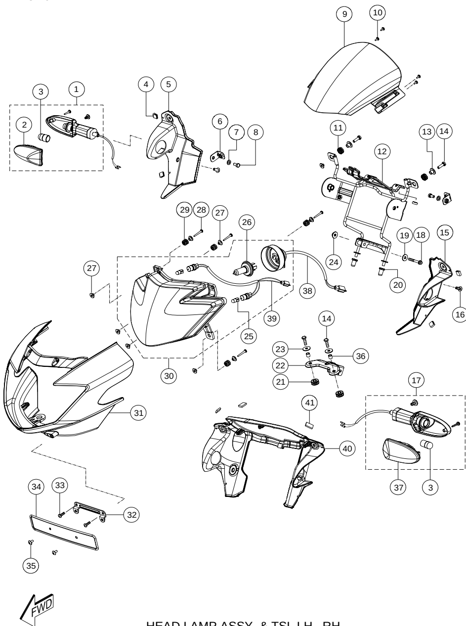
HEAD LAMP ASSY. &amp; TSL LH, RH
