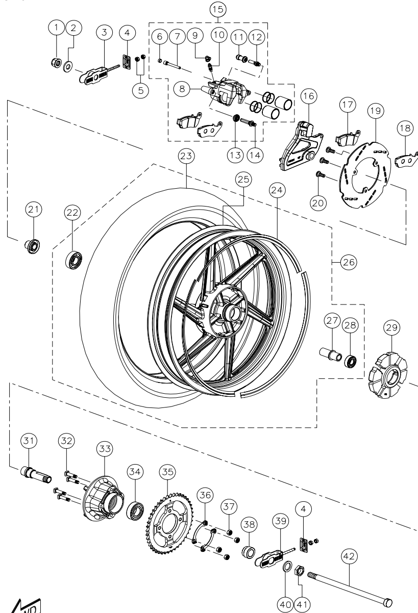
REAR WHEEL ASSEMBLY - DISC
