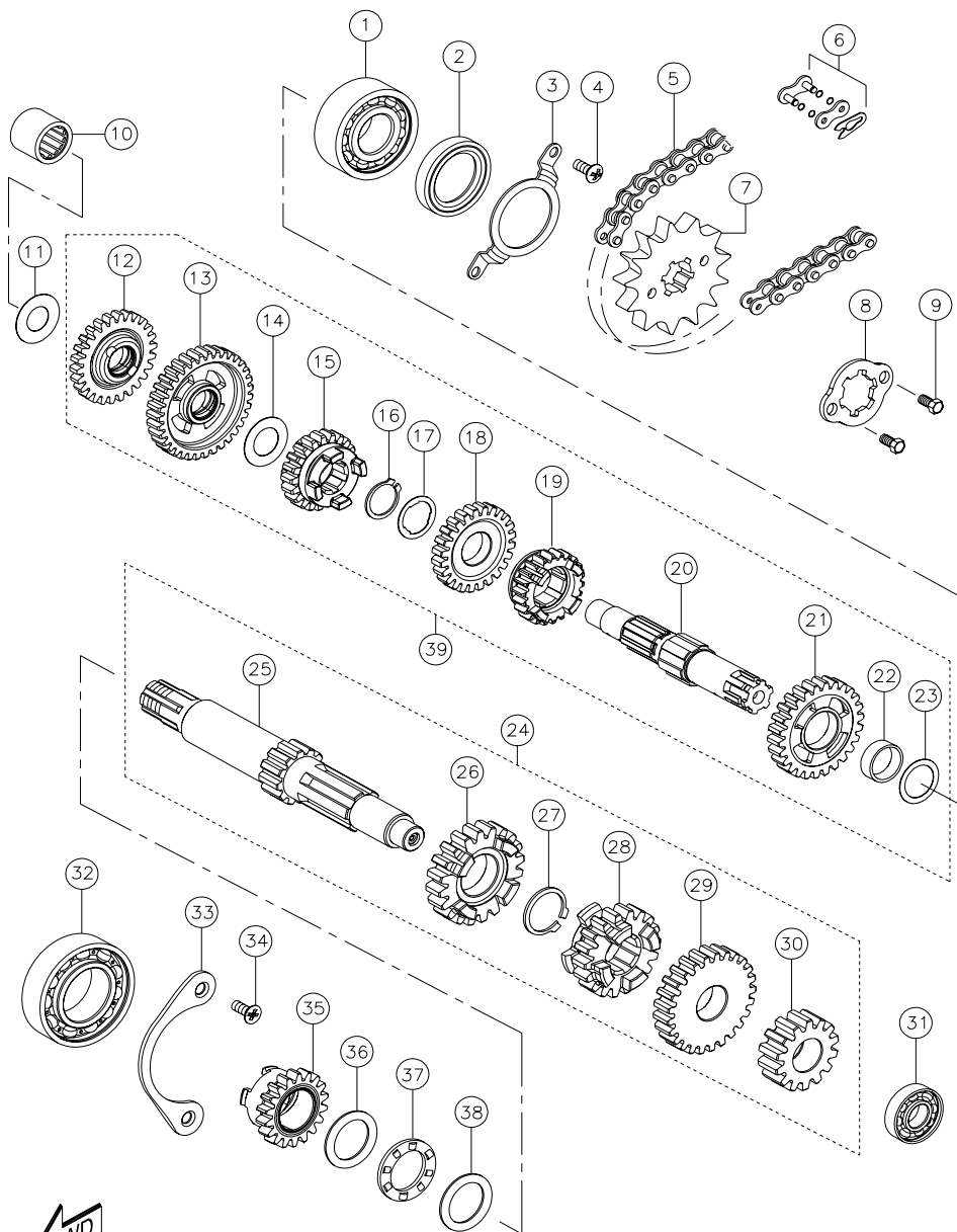
TRANSMISSION ASSEMBLY
