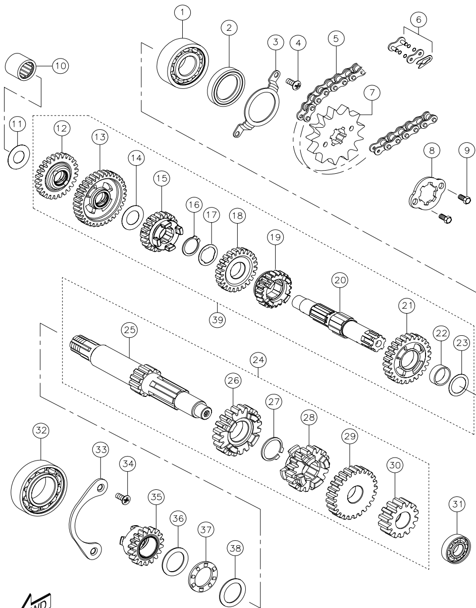
TRANSMISSION ASSEMBLY
