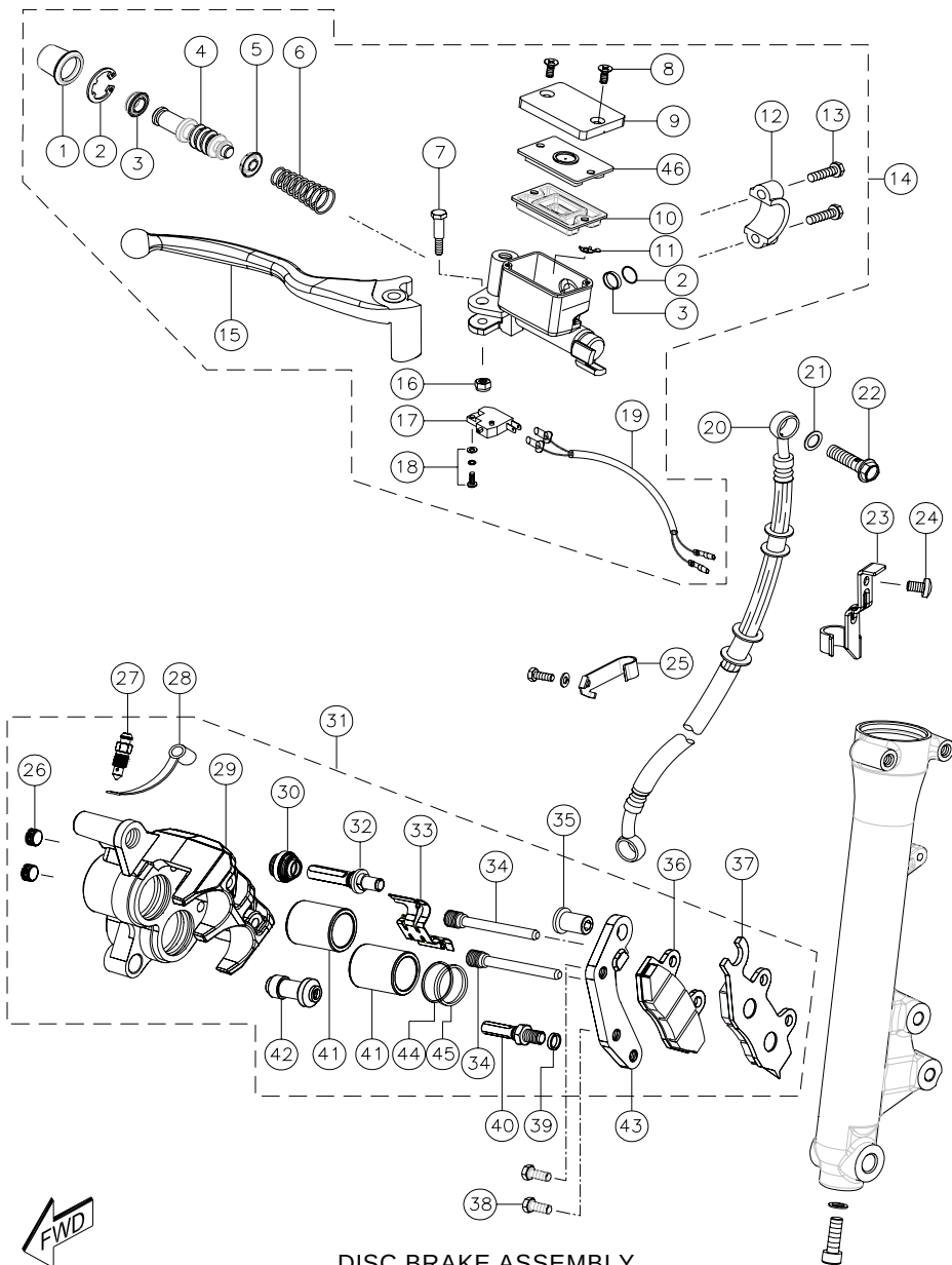
DISC BRAKE ASSEMBLY
