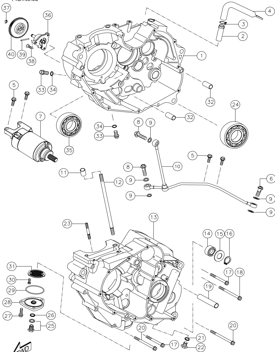
CRANKCASE LH, RH &amp; OIL PUMP ASSY.
