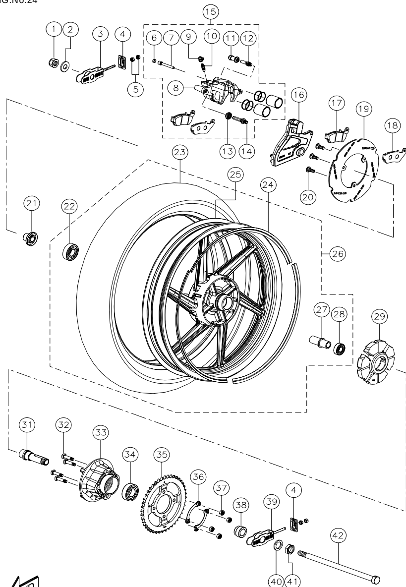
REAR WHEEL ASSEMBLY - DISC
