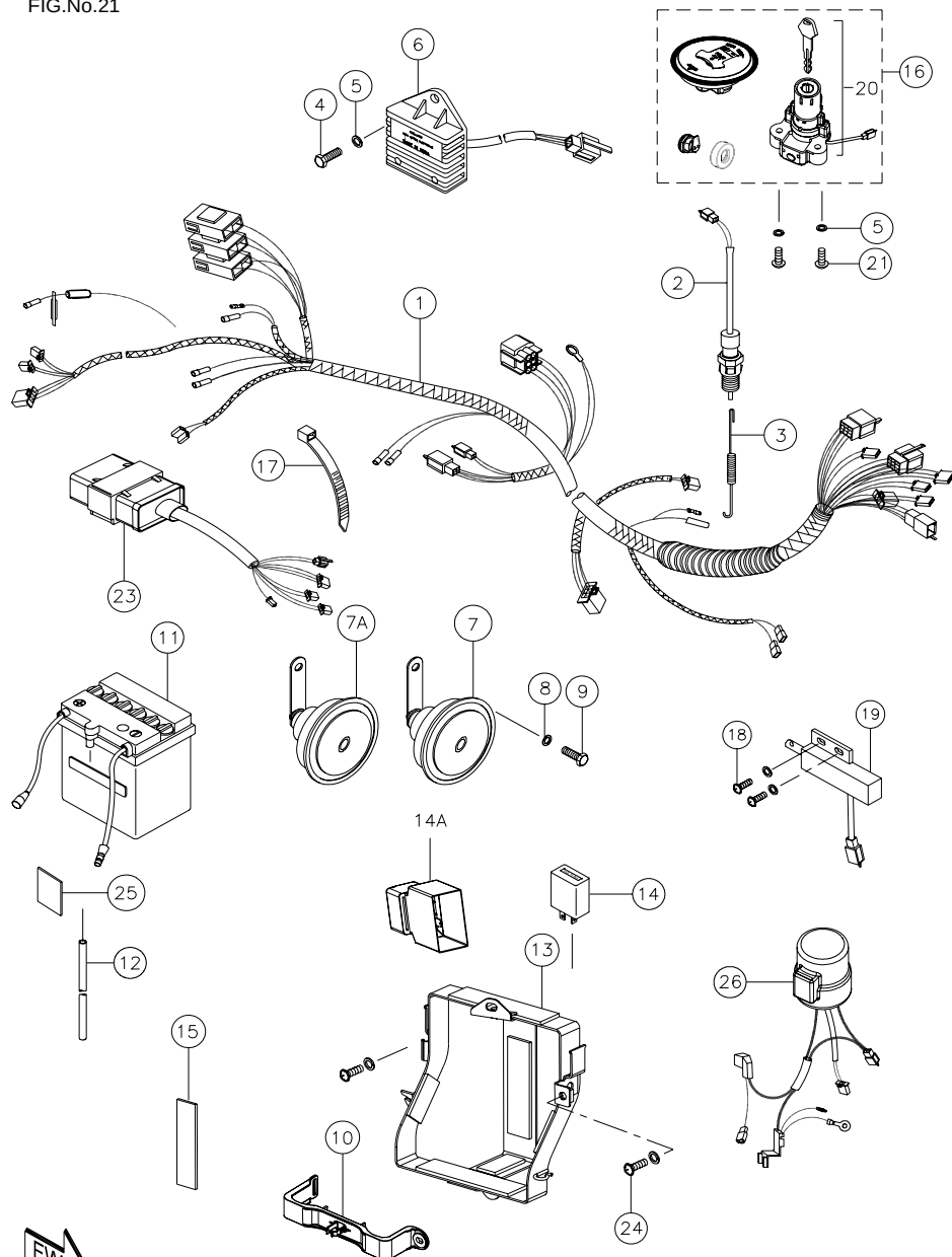
WIRING HARNESS, CDI UNIT &amp; BATTERY ASSEMBLY
