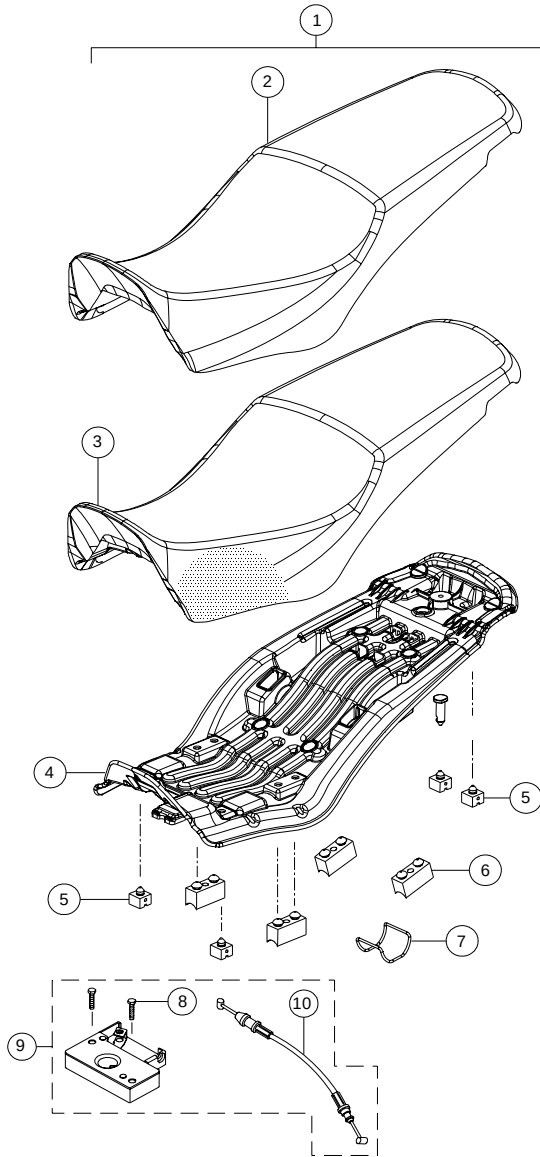
SEAT ASSEMBLY
