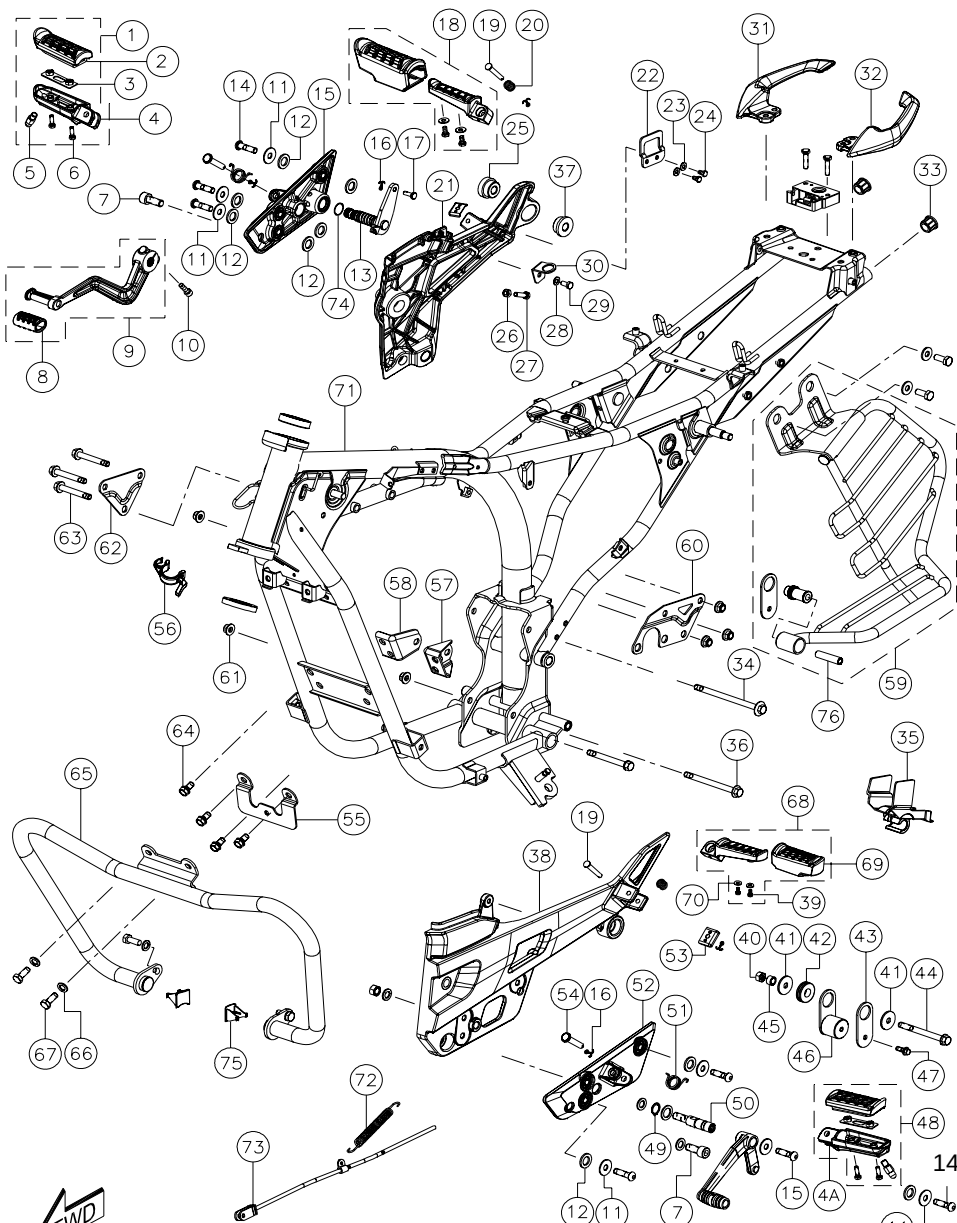
FRAME & SAREE GUARD ASSEMBLY
