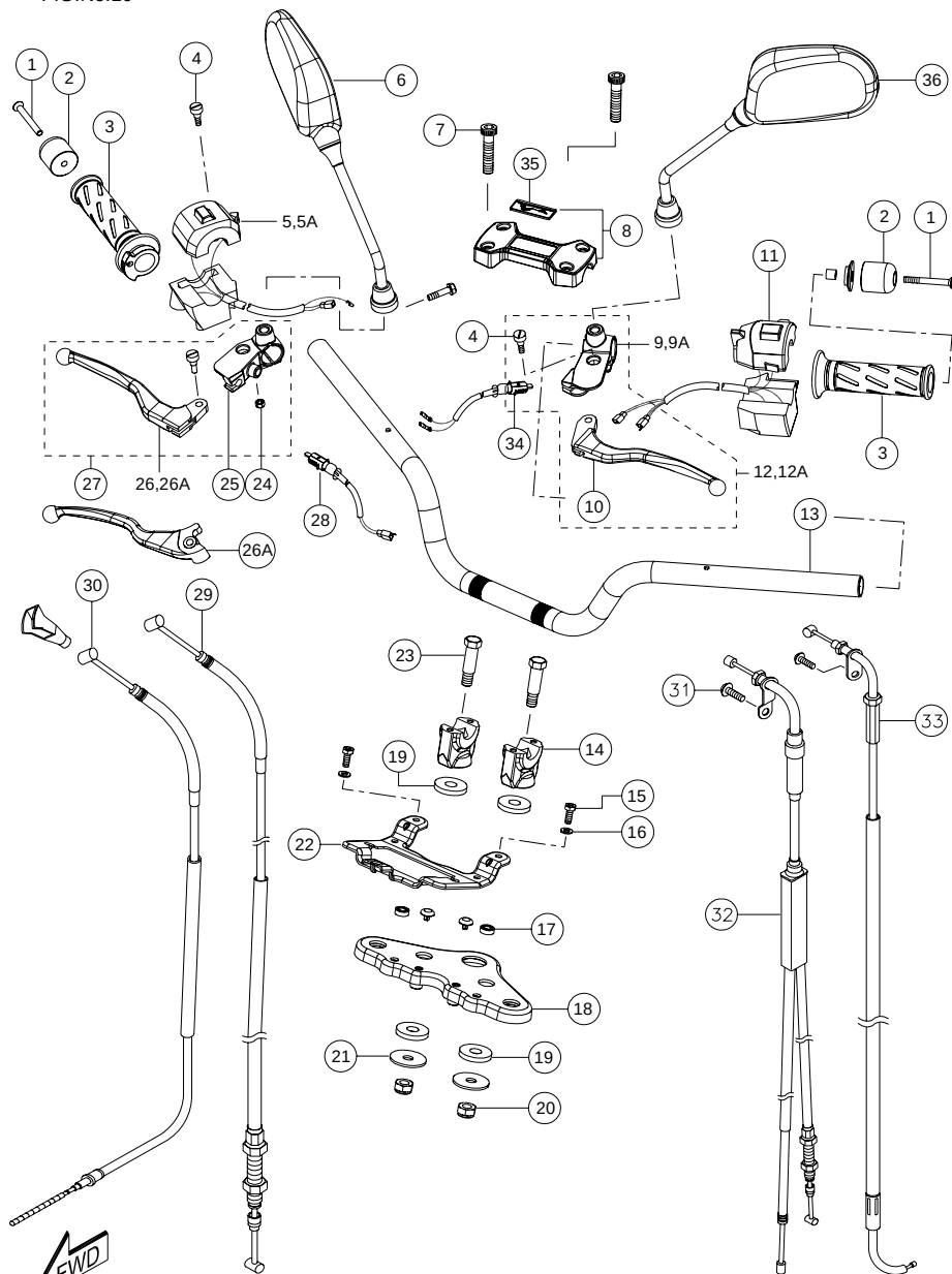
HANDLE BAR &amp; CABLE ASSY. (APACHE)
