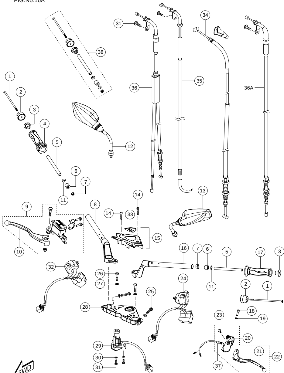
HANDLE BAR &amp; CABLE ASSY. (APACHE RTR)
