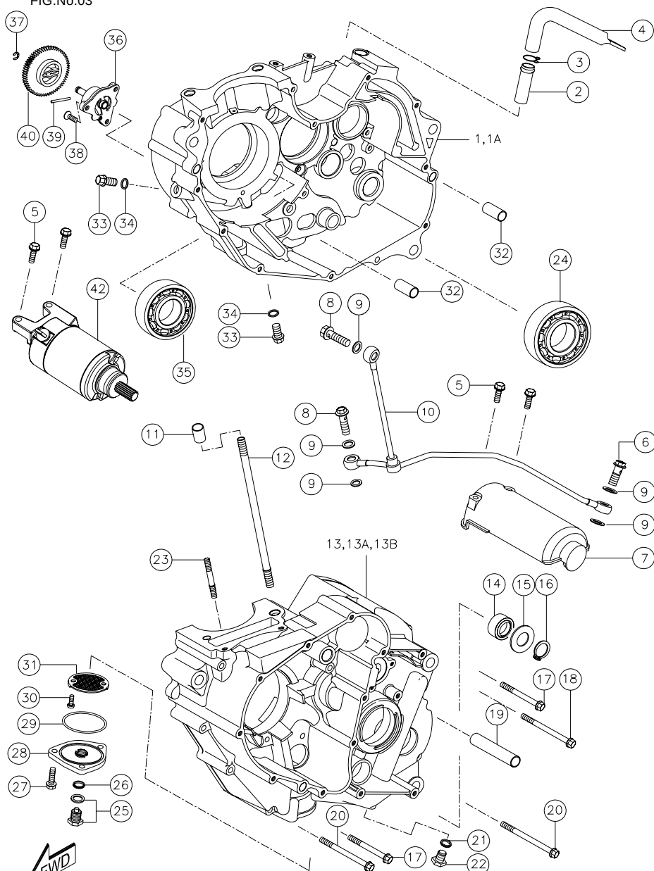
CRANKCASE LH, RH &amp; OIL PUMP ASSY.
