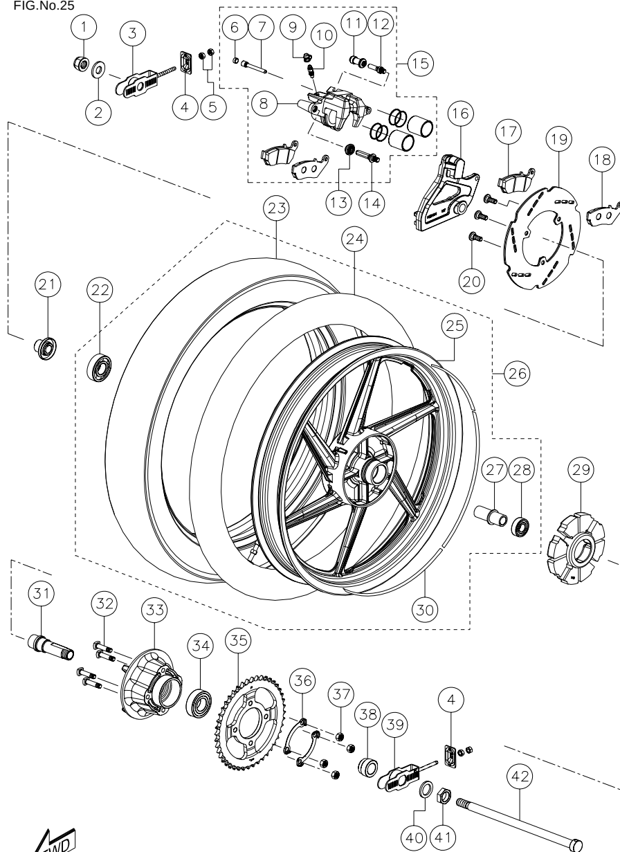
REAR WHEEL ASSEMBLY - EFI (DISC)
