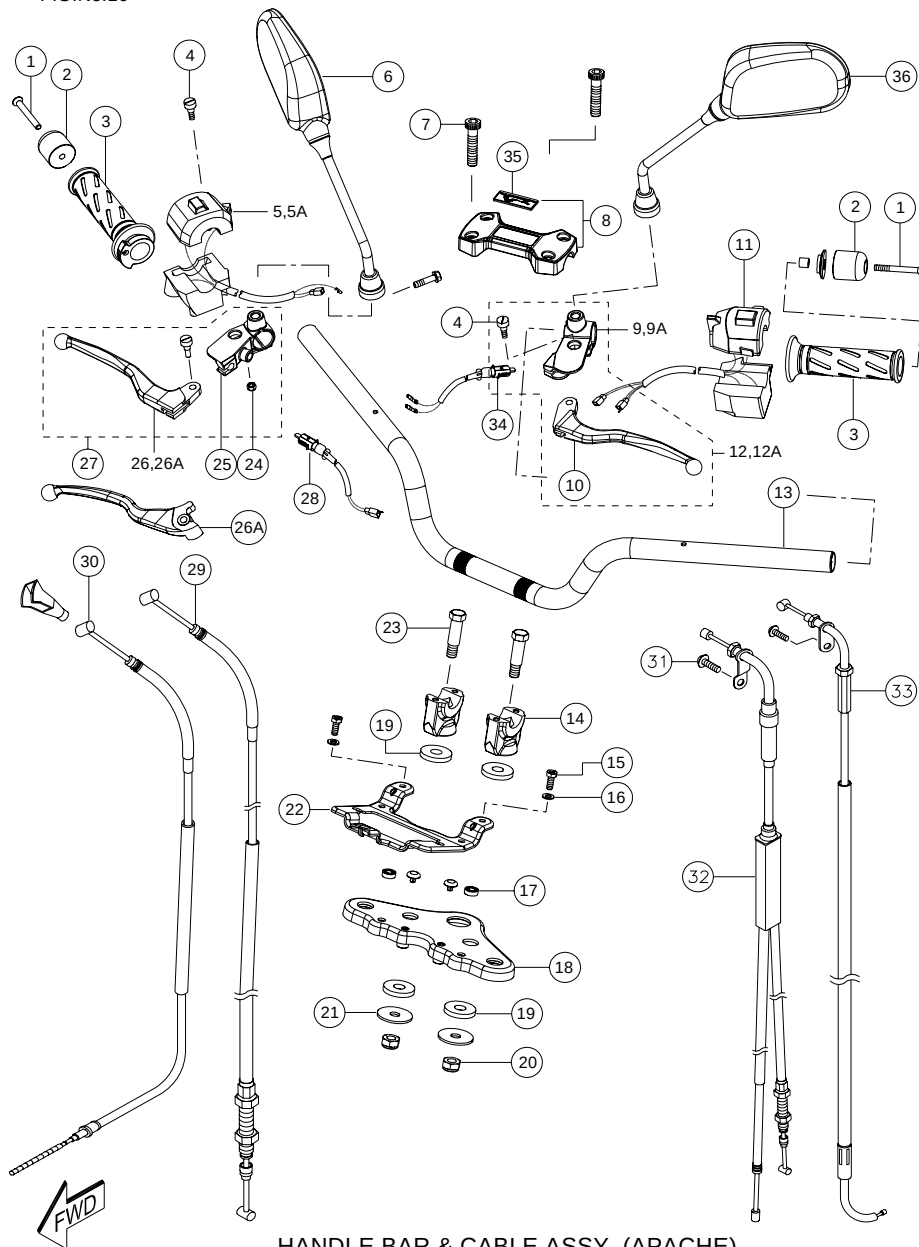
HANDLE BAR &amp; CABLE ASSY. (APACHE)
