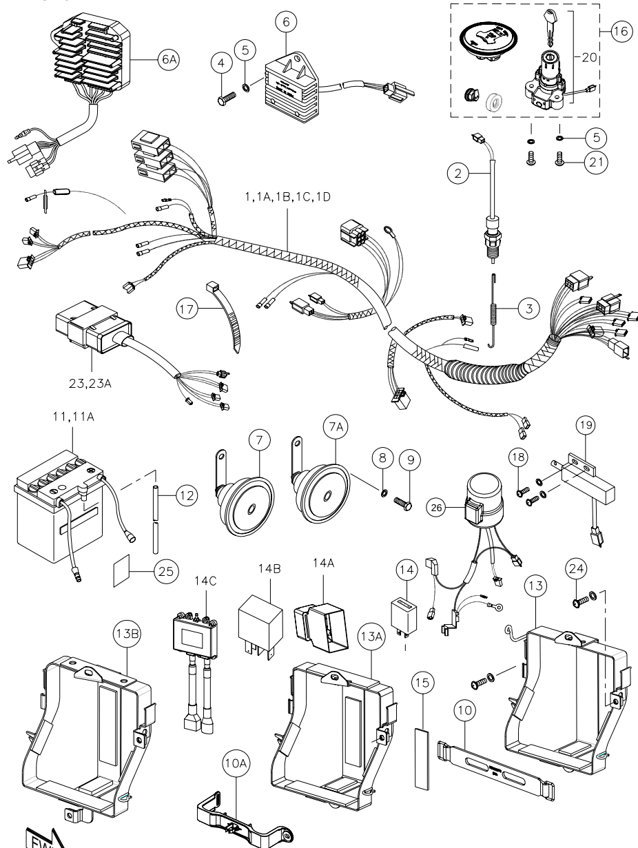
WIRING HARNESS, CDI UNIT &amp; BATTERY ASSEMBLY
