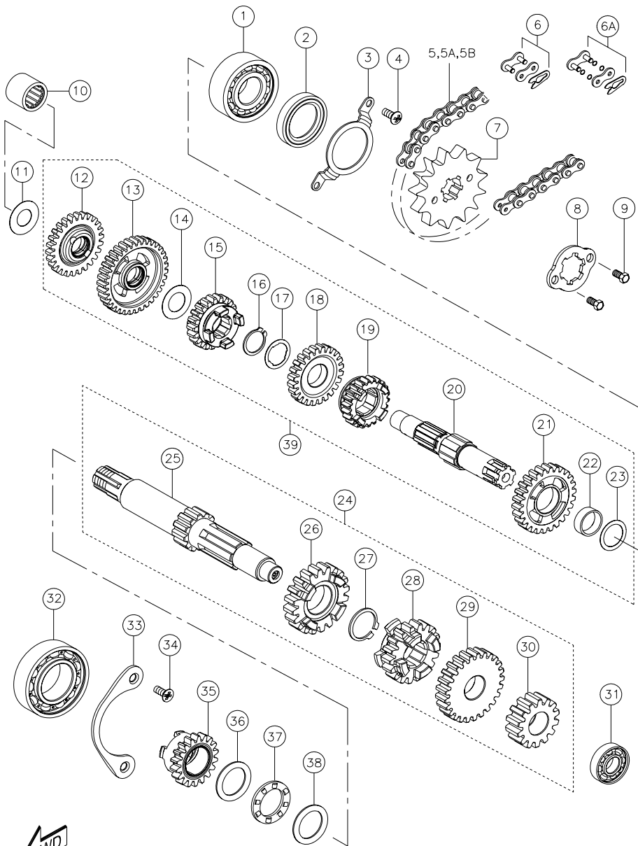
TRANSMISSION ASSEMBLY
