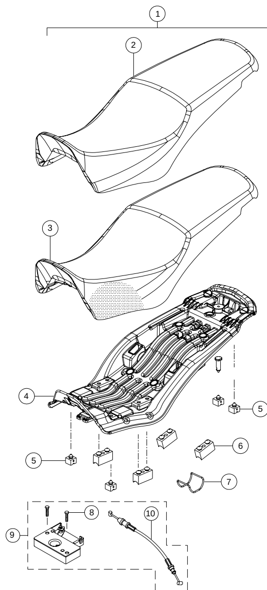
SEAT ASSEMBLY
