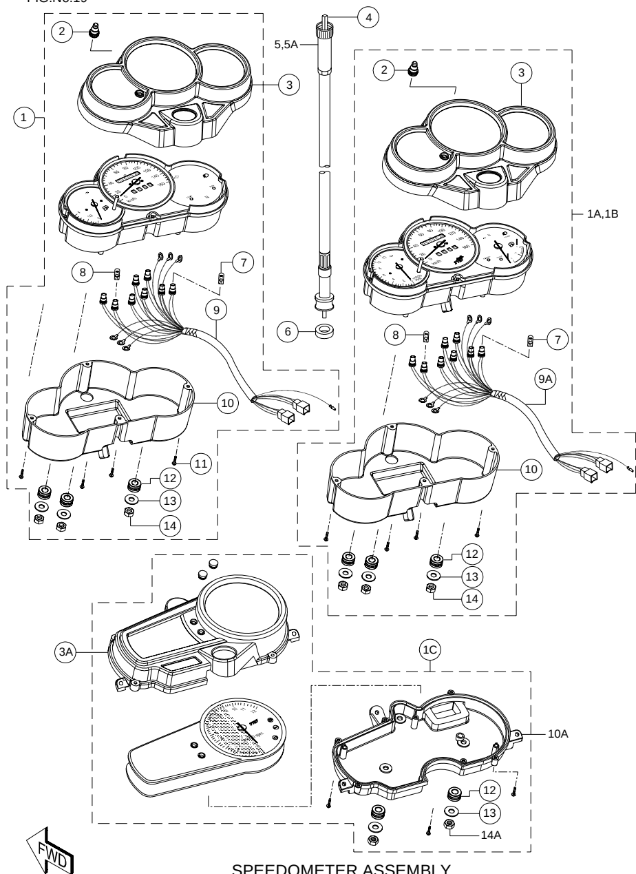
SPEEDOMETER ASSEMBLY
