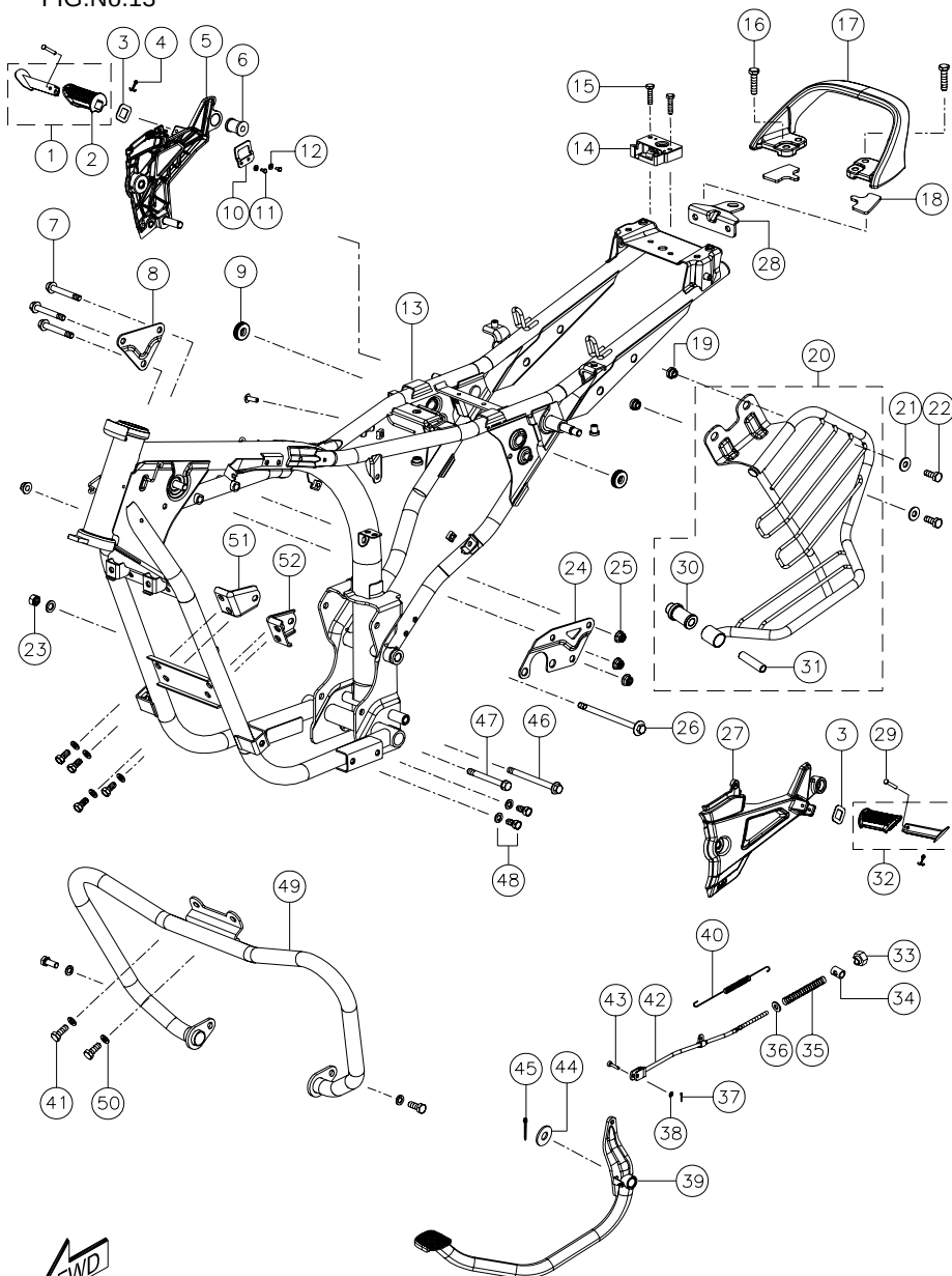
FRAME &amp; SAREE GUARD ASSEMBLY (APACHE)
