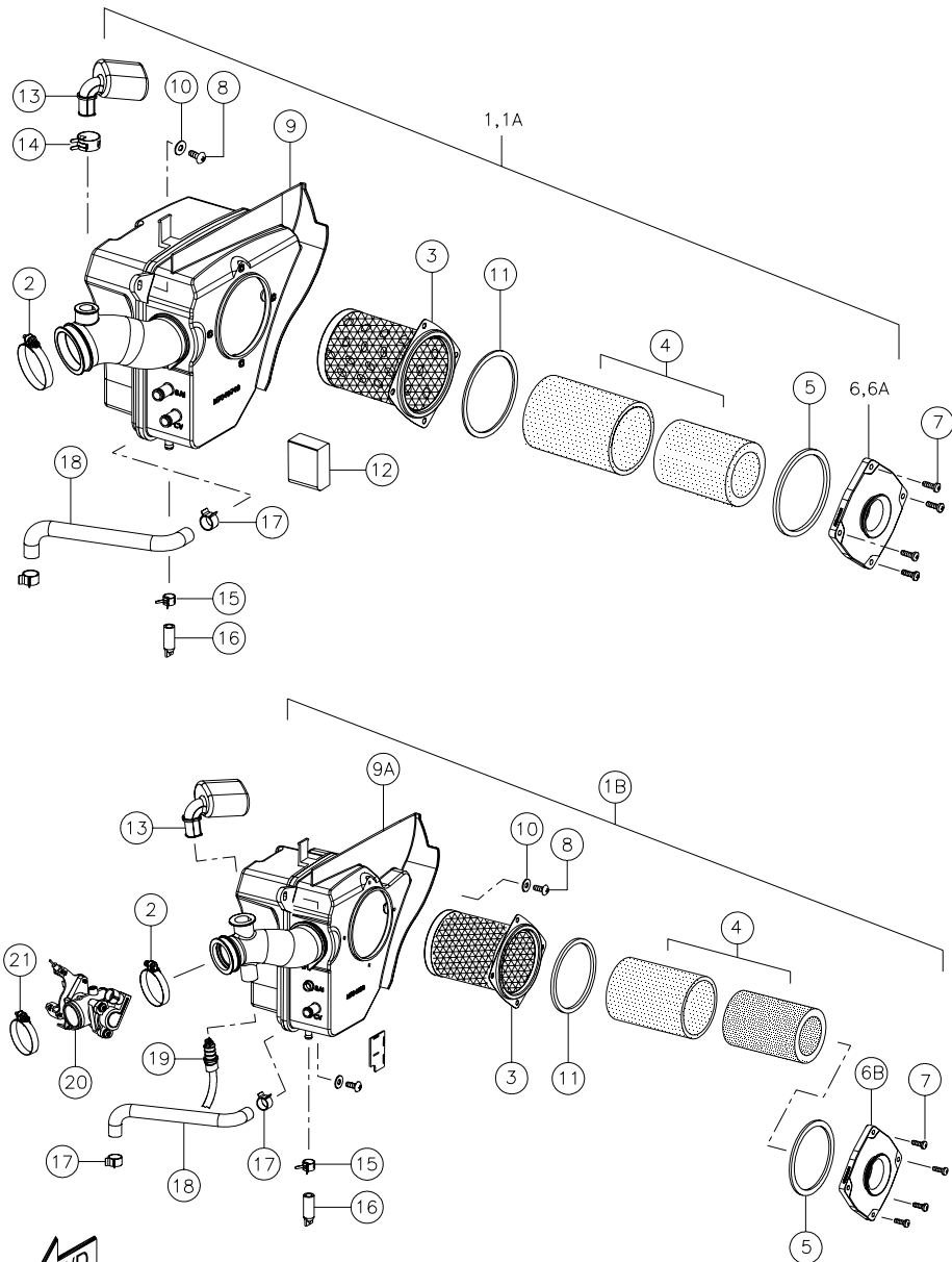
AIR CLEANER ASSEMBLY
