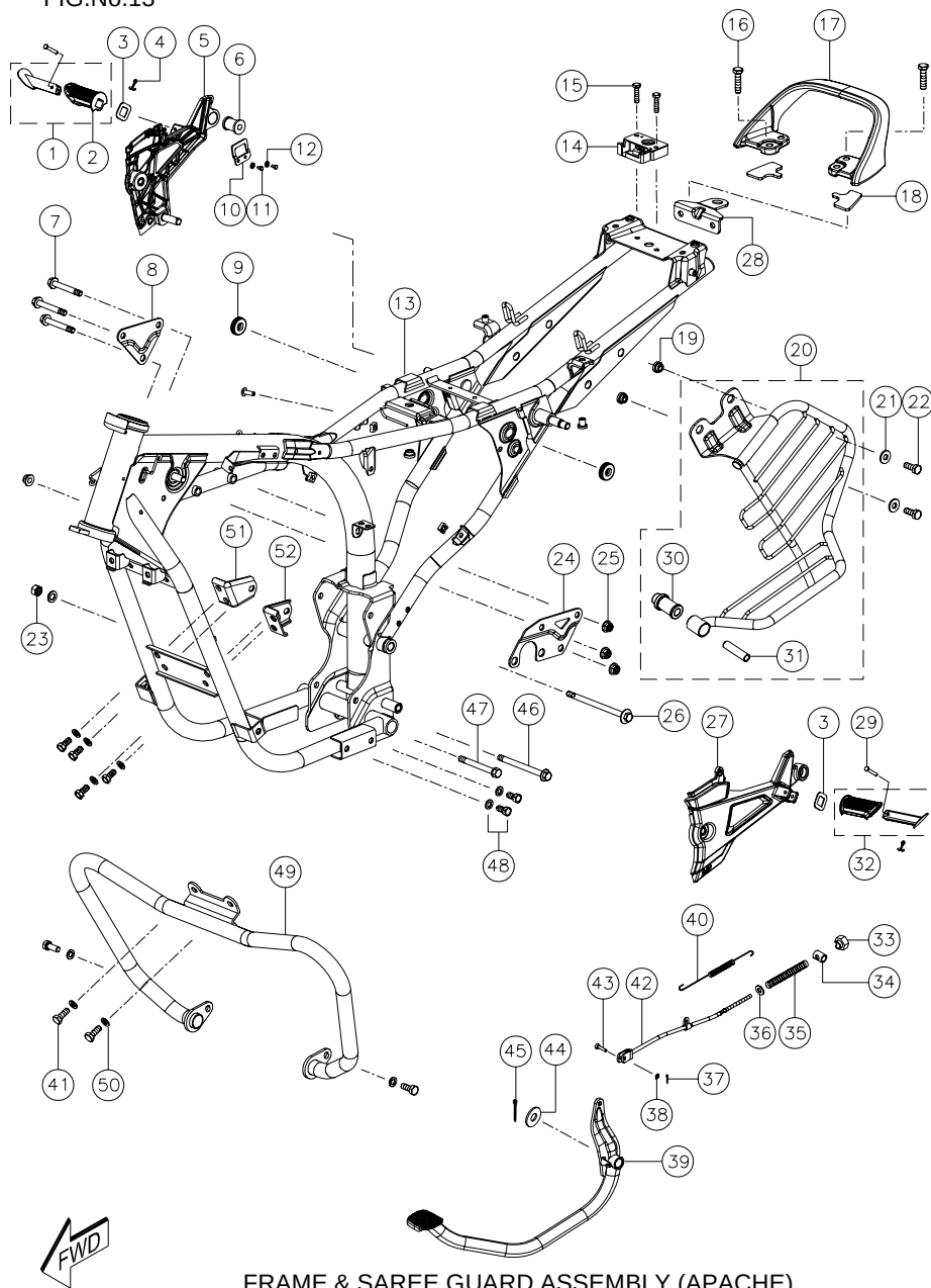
FRAME &amp; SAREE GUARD ASSEMBLY (APACHE)
