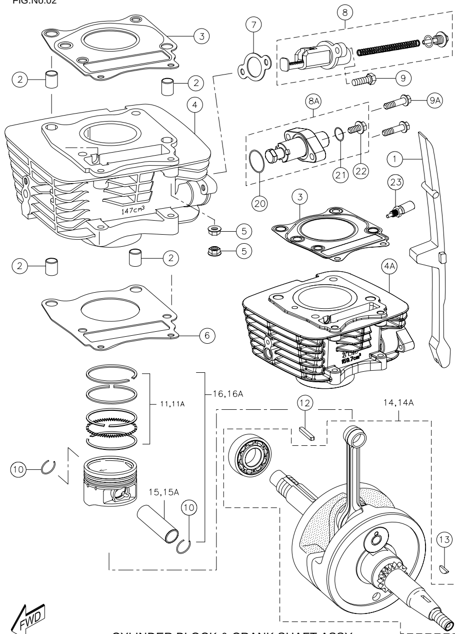
CYLINDER BLOCK &amp; CRANK SHAFT ASSY.
