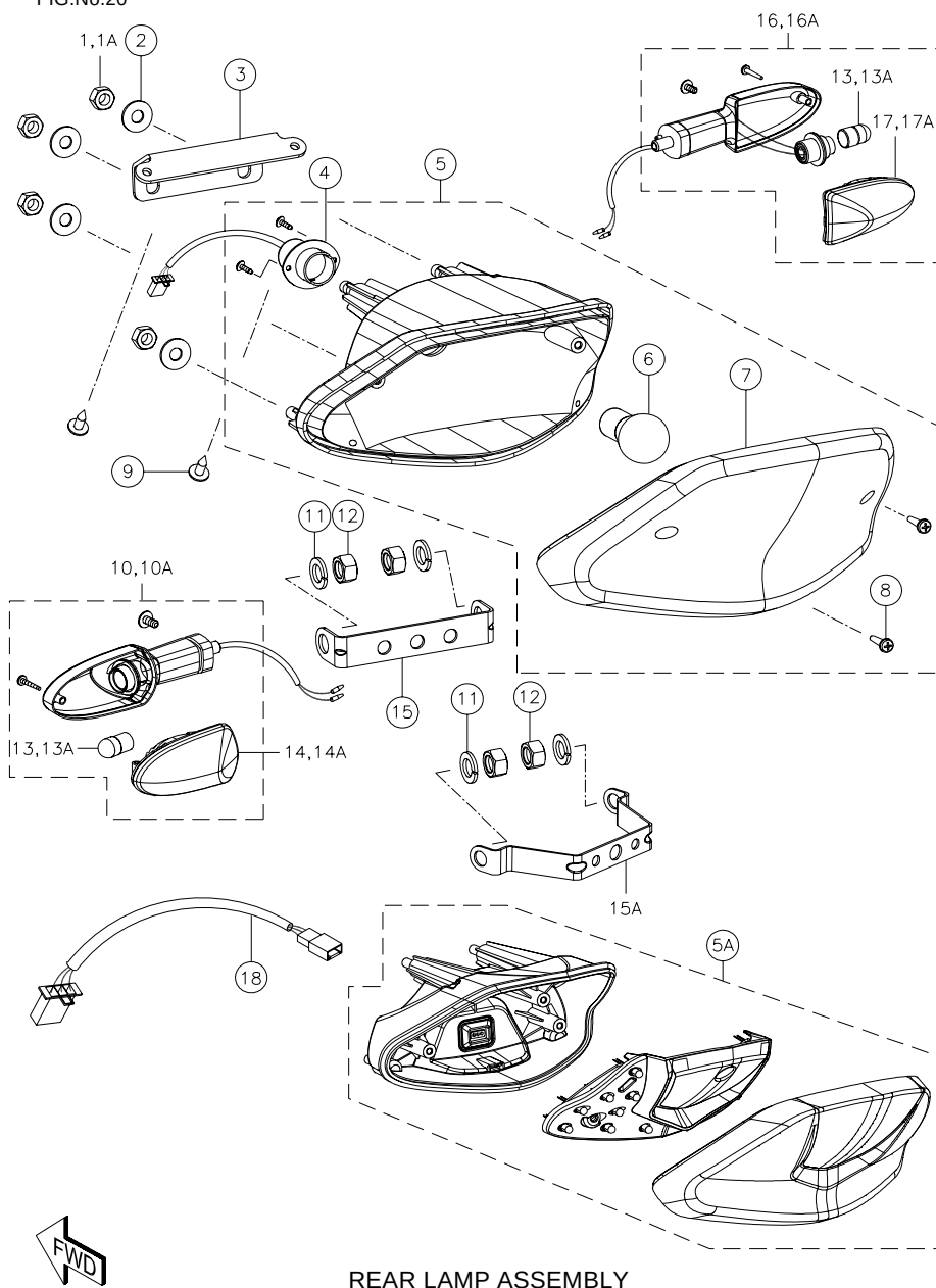
REAR LAMP ASSEMBLY
