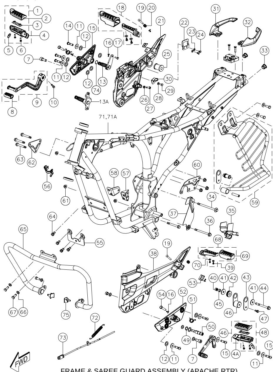
FRAME &amp; SAREE GUARD ASSEMBLY (APACHE RTR)
