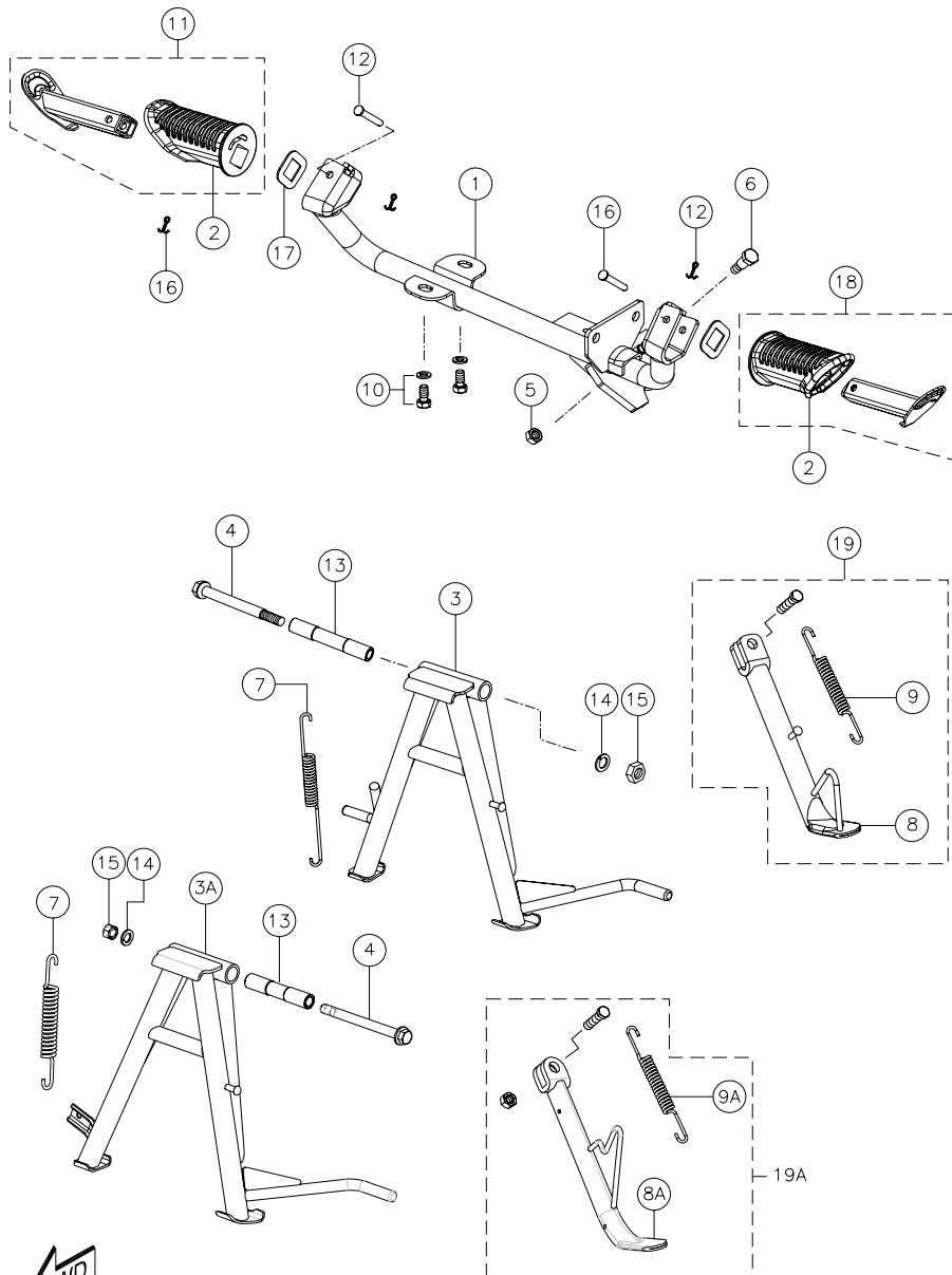
CENTER STAND &amp; FOOTREST ASSEMBLY
