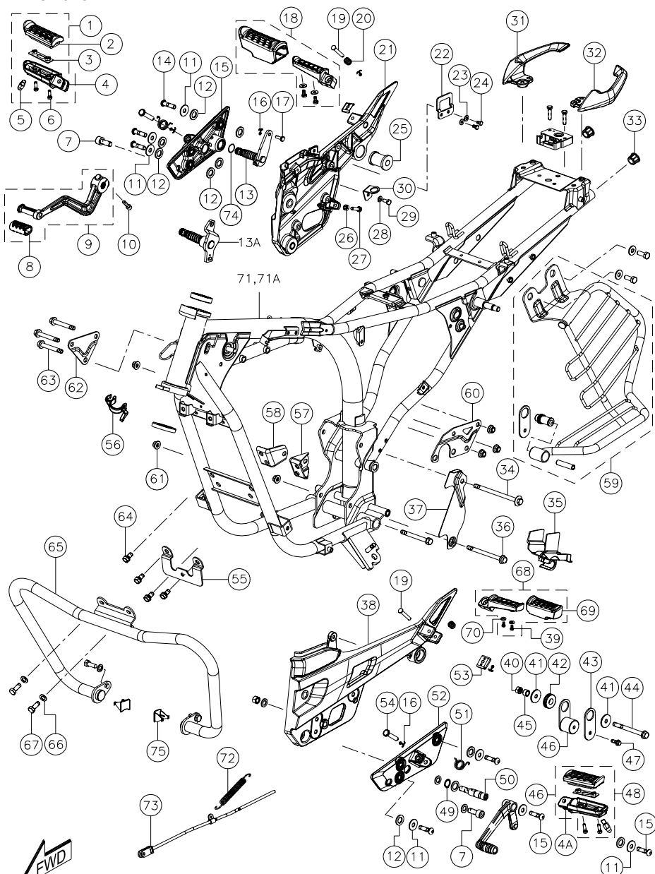
FRAME &amp; SAREE GUARD ASSEMBLY (APACHE RTR)
