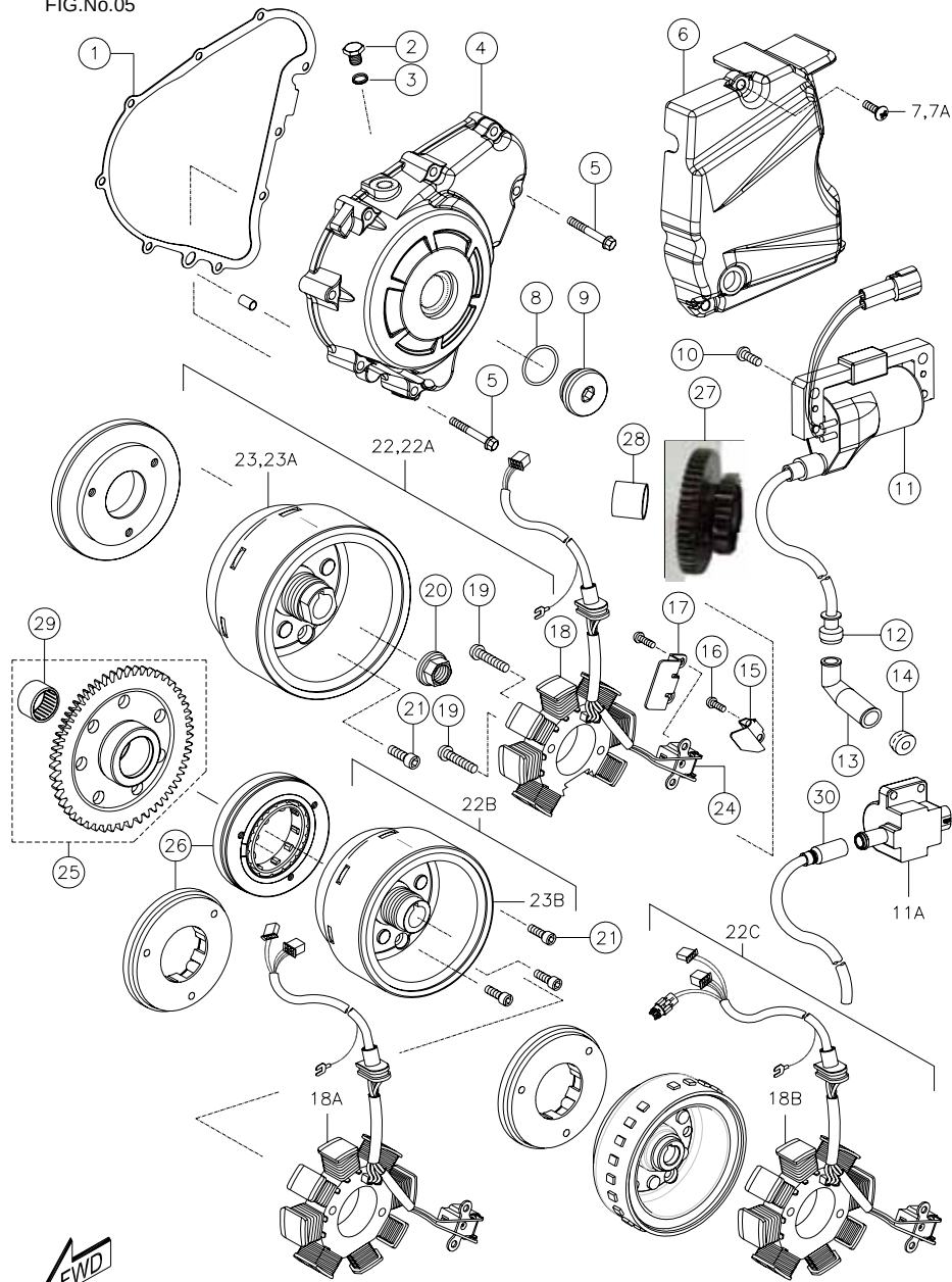
MAGNETO &amp; IGNITION COIL ASSEMBLY
