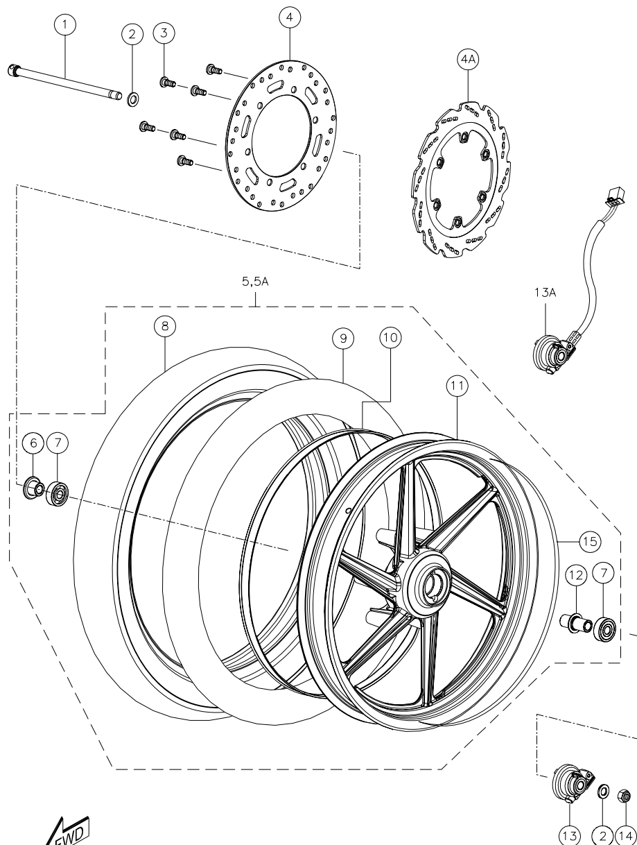
FRONT ALLOY WHEEL ASSY. (DISC BRAKE)
