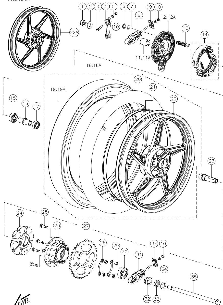
REAR WHEEL ASSEMBLY (ALLOY)
