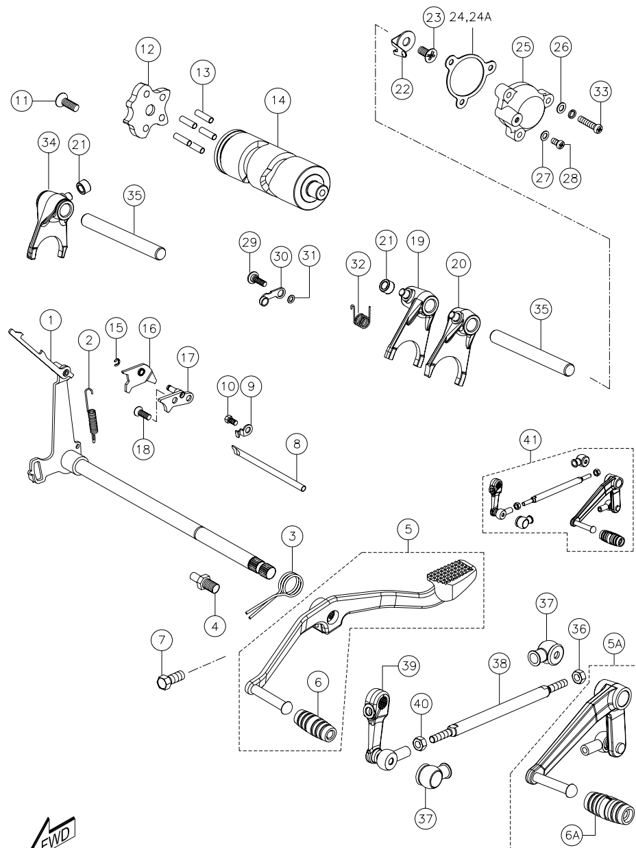
GEAR SHIFT MECHANISM ASSEMBLY
