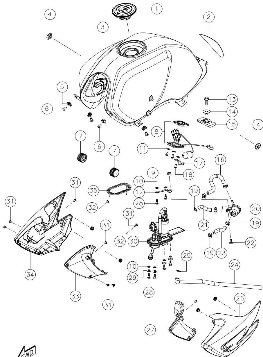
FUEL TANK &amp; FUEL PUMP ASSY. EFI
