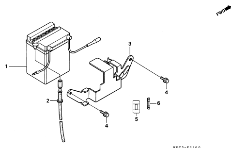
C-27 Chassi / Frame / Chasis
