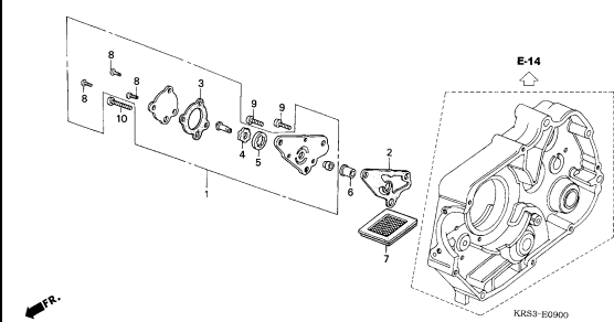
OIL PUMP
