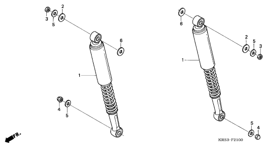
REAR CUSHION
