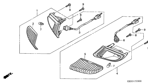
WINKER (NF100M3/MSH3)
