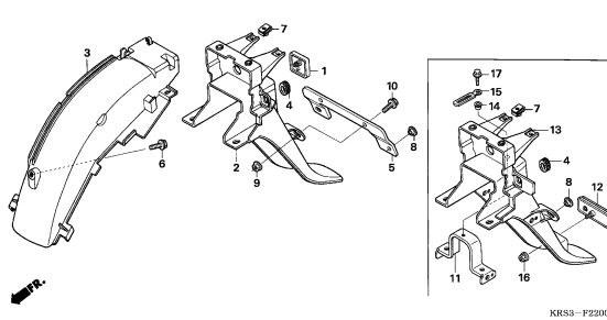
REAR FENDER
