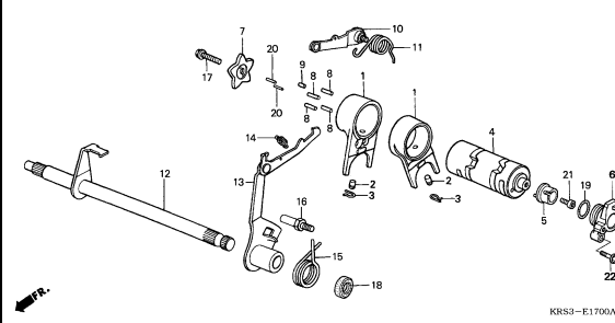
GEARSHIFT DRUM
