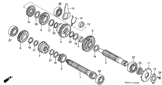
TRANSMISSION
