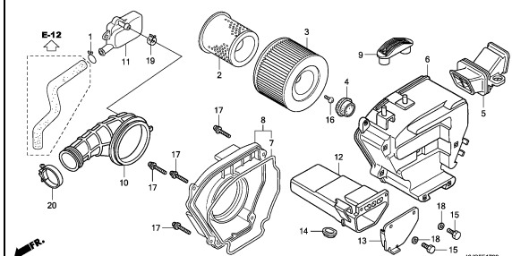
AIR CLEANER
