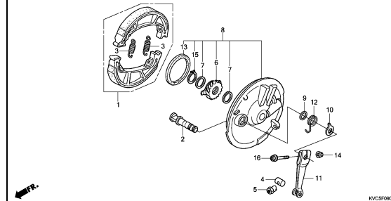
FRONT BRAKE PANEL
