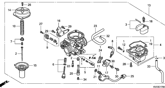
CARBURETOR
