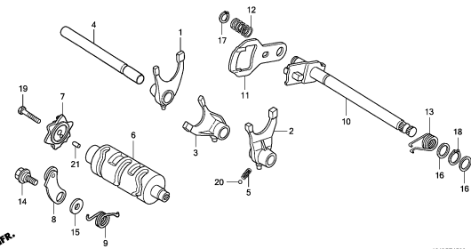
GEARSHIFT DRUM
