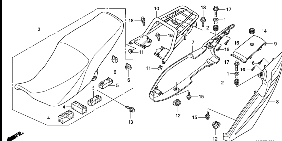
SEAT/REAR COWL
