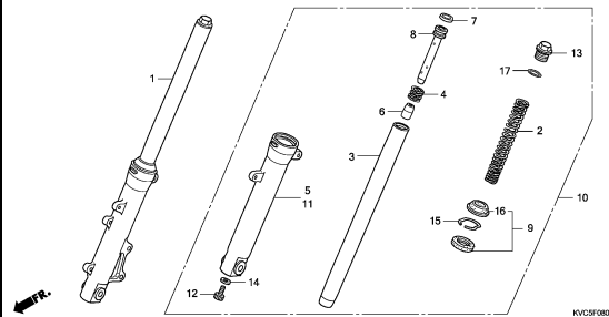
FRONT FORK
