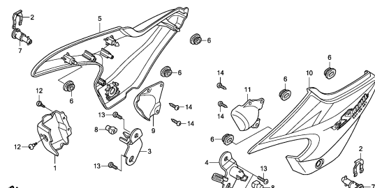
SIDE COVER
