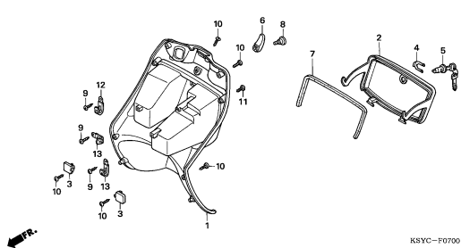
INNER BOX
