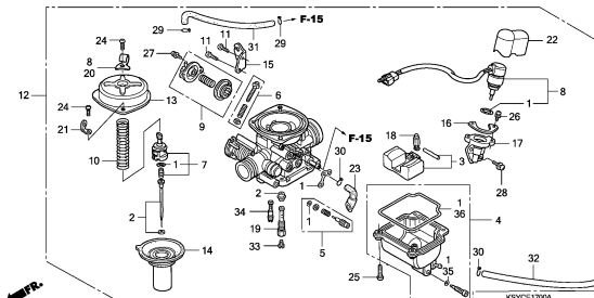
CARBURETOR
