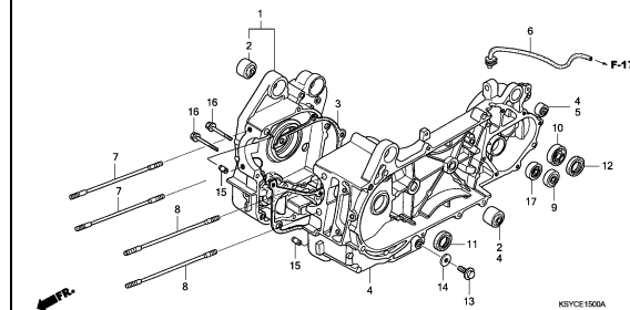
CRANKCASE
