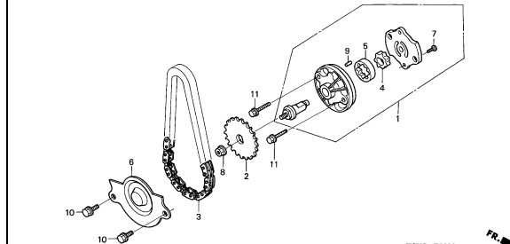
OIL PUMP
