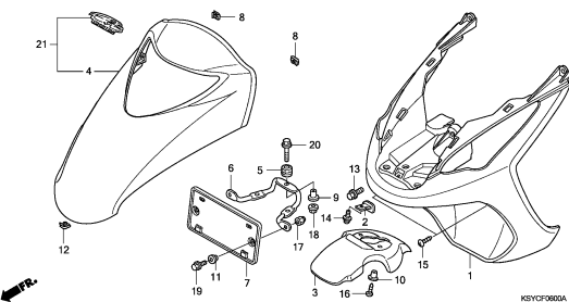
FRONT COVER
