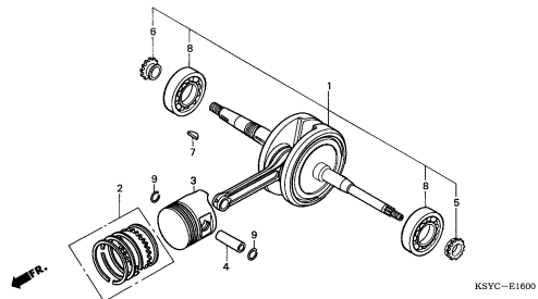
CRANKSHAFT/PISTON
