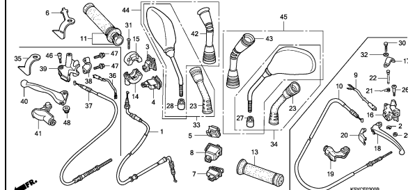
STEERING HANDLE/HANDLE COVER(2)
