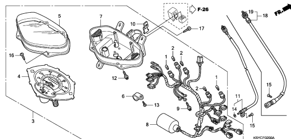
STEERING HANDLE/HANDLE COVER(1)
